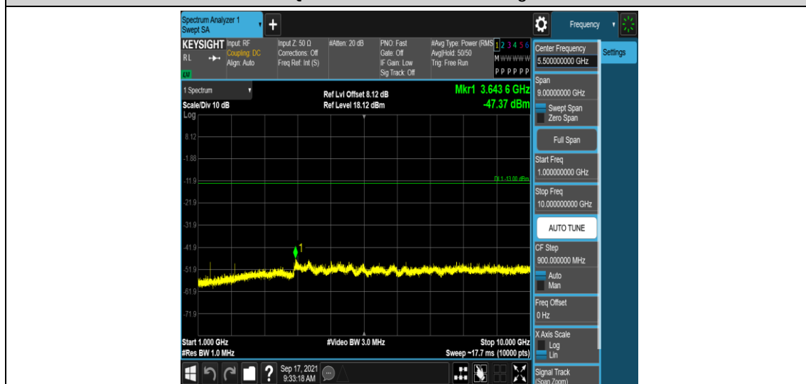
Band71-15MHz-QPSK-133197-1RB#0-Range4:1000~10000MHz
