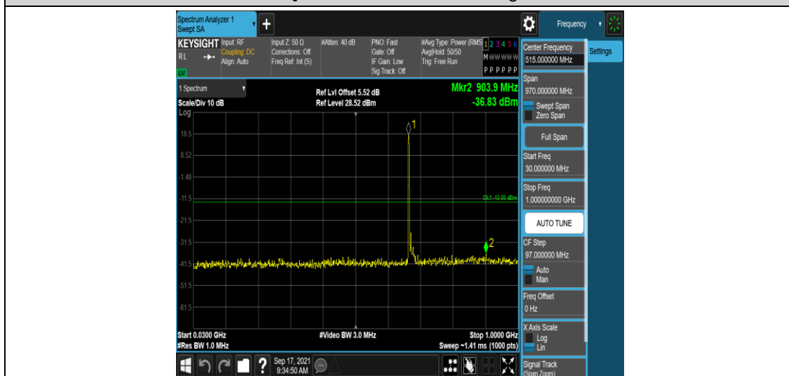
Band71-15MHz-QPSK-133297-1RB#0-Range3:30~1000MHz
