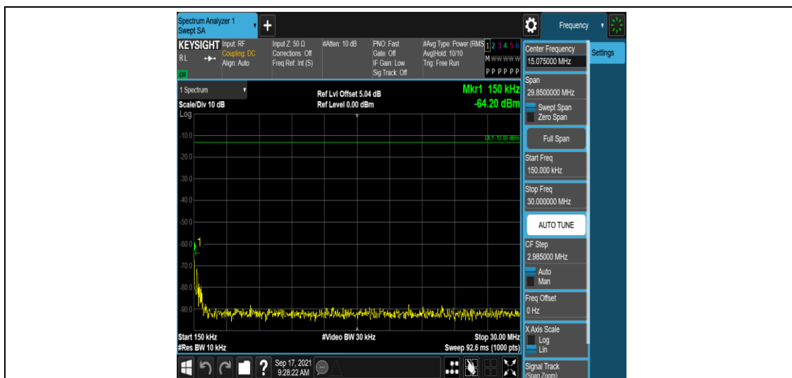
Band71-10MHz-16QAM-133172-1RB#0-Range2:0.15~30MHz
