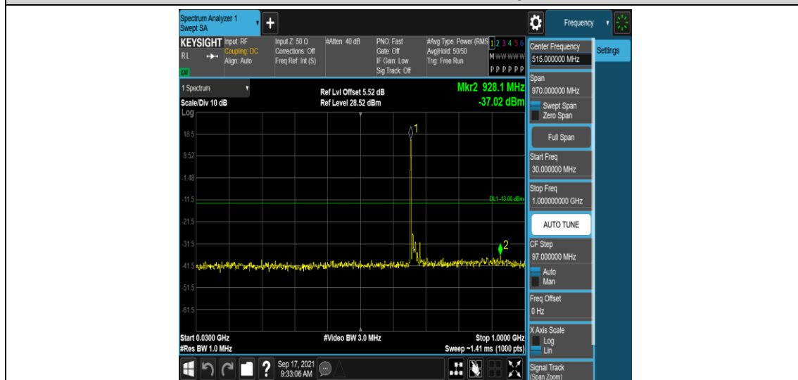
Band71-15MHz-QPSK-133197-1RB#0-Range3:30~1000MHz
