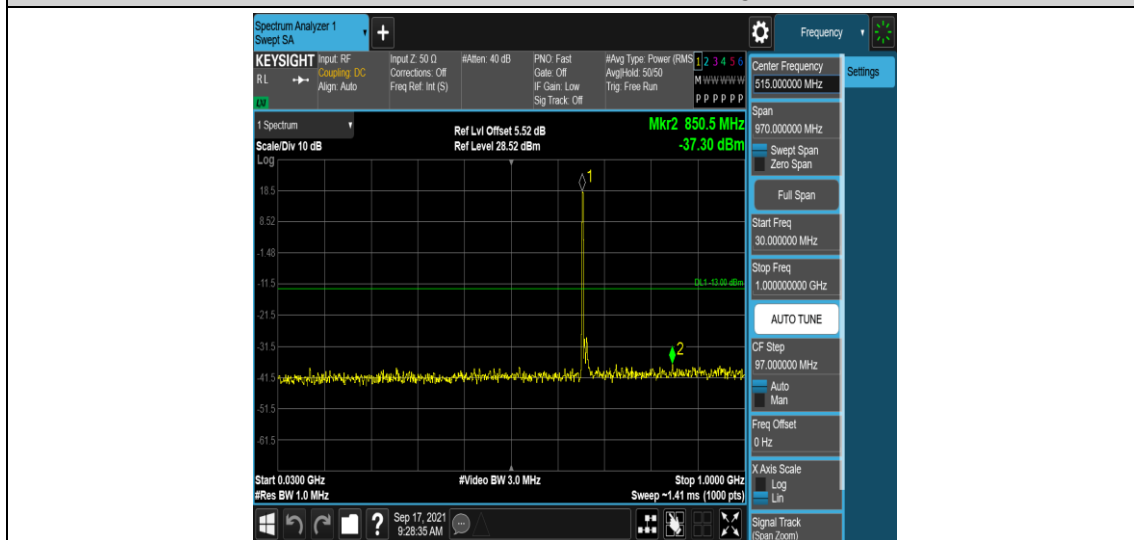
Band71-10MHz-16QAM-133172-1RB#0-Range3:30~1000MHz
