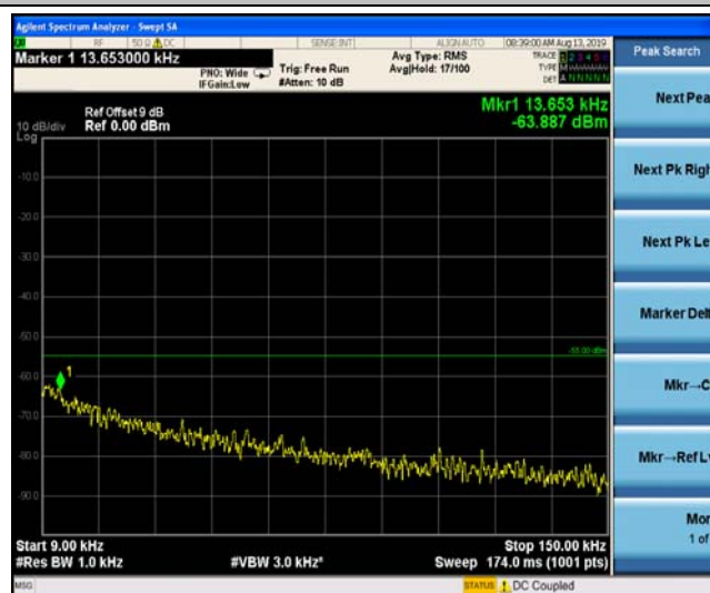
Band41_5MHz_16QAM_40620_1RB#0
