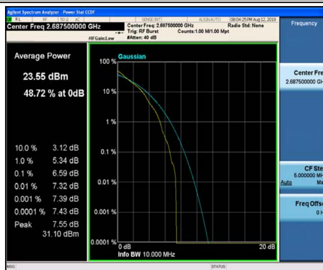
Band41_5MHz_QPSK_41565_25RB#0
