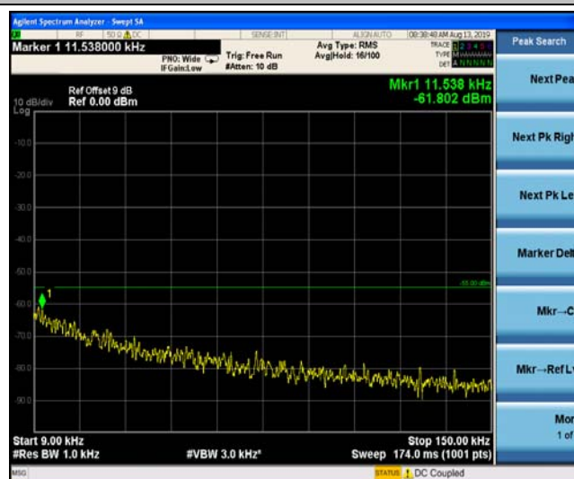
Band41_5MHz_QPSK_40620_1RB#0
