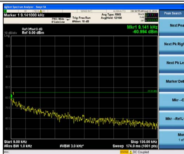
Band41_5MHz_16QAM_39675_1RB#0
