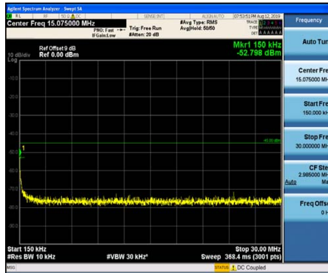
Band41_5MHz_QPSK_39675_1RB#0
