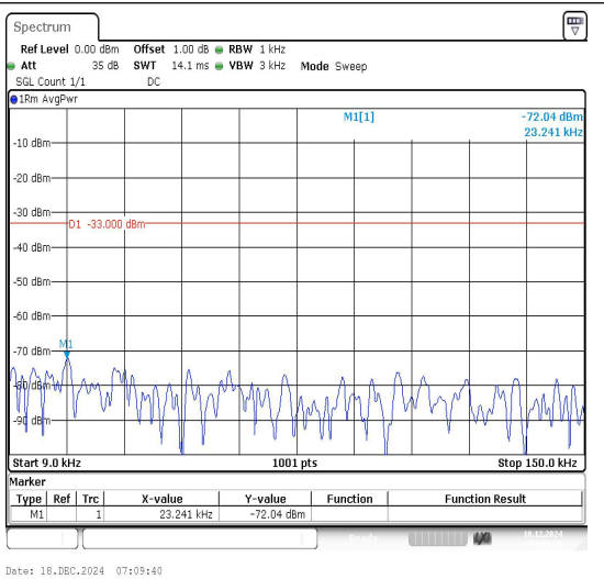
Band12_10MHz_16QAM_23060_1RB#0_0.009~0.15_0.009~0.15
