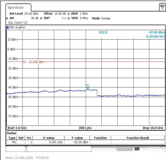
Band12_10MHz_QPSK_23060_1RB#0_3000~10000_3000~10000
