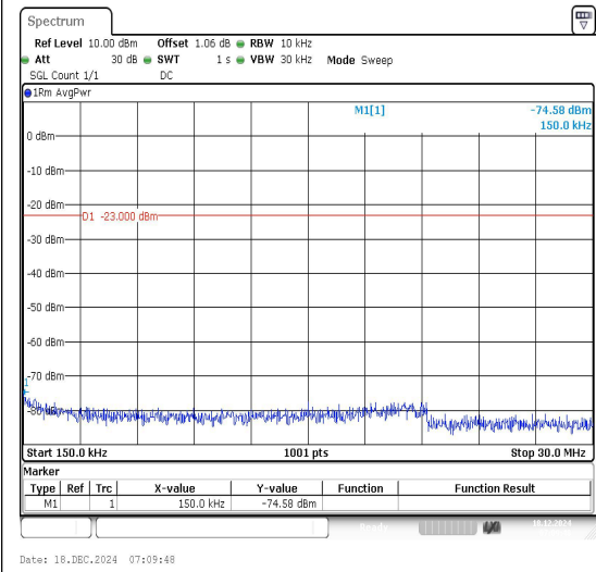
Band12_10MHz_QPSK_23060_1RB#0_3000~10000_0_0.15~30
