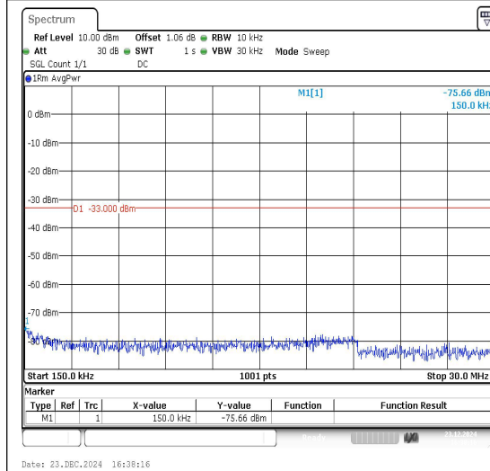
Band66_5MHz_16QAM_132647_1RB#0_0.15~30_0.15~30
