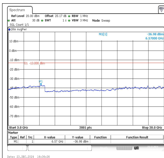
Band66_5MHz_QPSK_132322_1RB#0_3000~20000
