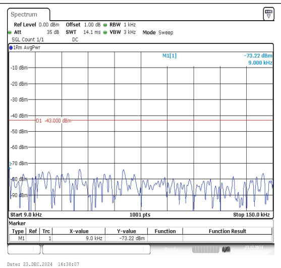
Band66_5MHz_16QAM_132647_1RB#0_0.009~0.15_0.009~0.15
