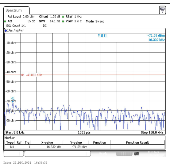
Band66_5MHz_16QAM_132322_1RB#0_0.009~0.15
