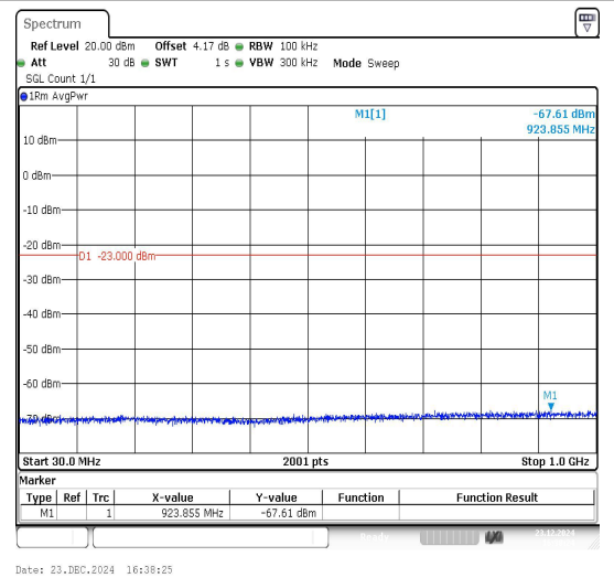
Band66_5MHz_16QAM_132647_1RB#0_30~1000_30~1000
