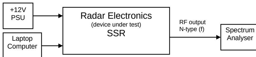
Figure 2 Test Configuration – Conducted Spurious Emissions Test
