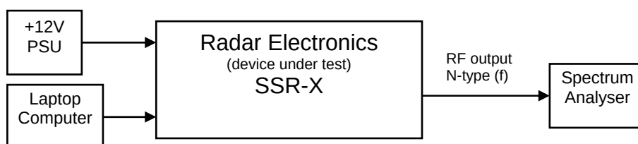
Figure 2 Test Configuration – Conducted Spurious Emissions Test
