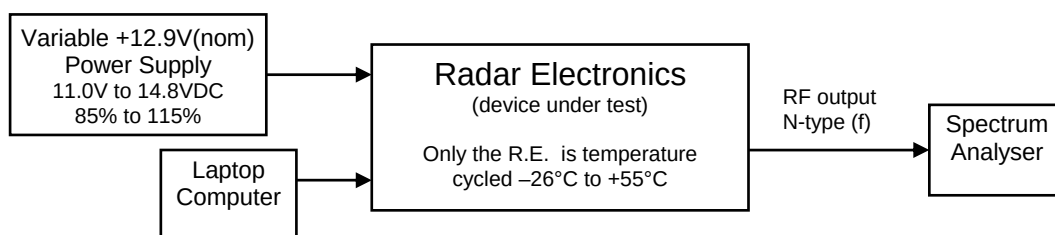
Figure 3 Test Configuration – Frequency Stability Test
