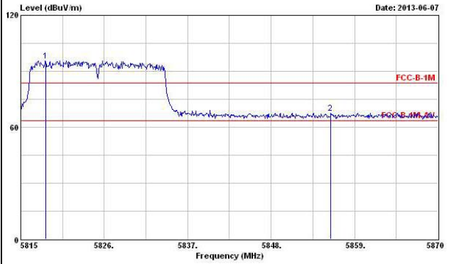
HT40-(Highest Ch.)
