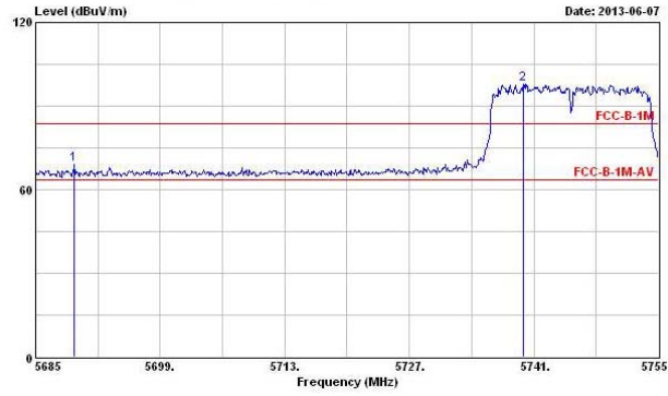
HT40-(Lowest Ch.)
