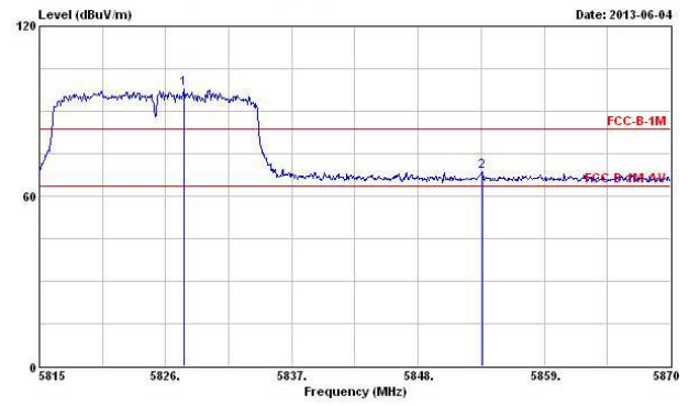
HT40-(Highest Ch.)
