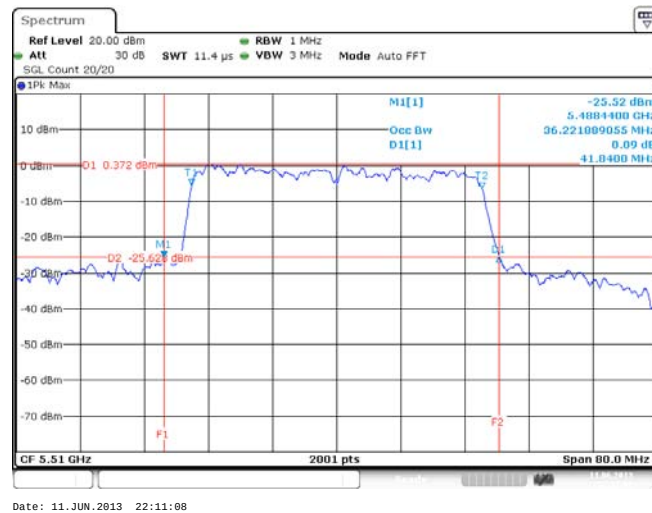
HT40
