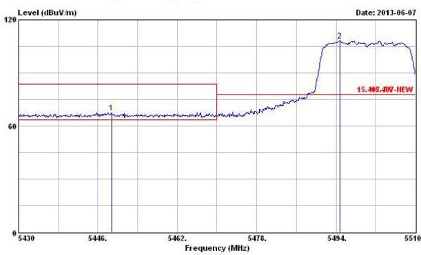
HT40,M8-15-(Lowest Ch.)
