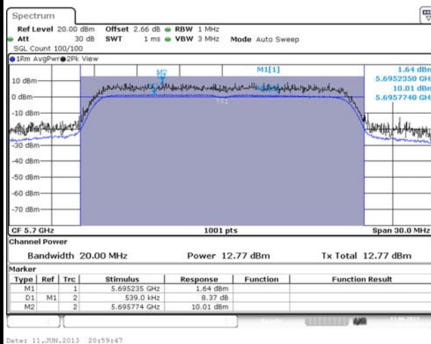
HT20 [Port 2]
