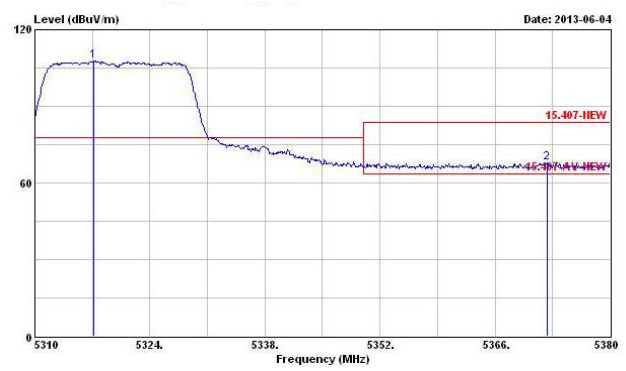
HT40,M16-23-(Highest Ch.)
