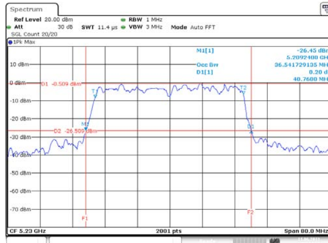
HT40
