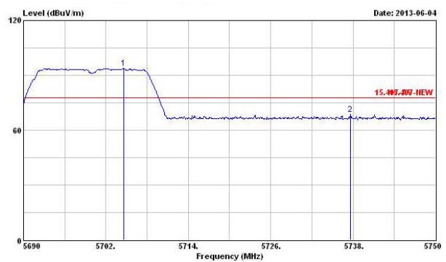
HT20,M8-15-(Highest Ch.)
