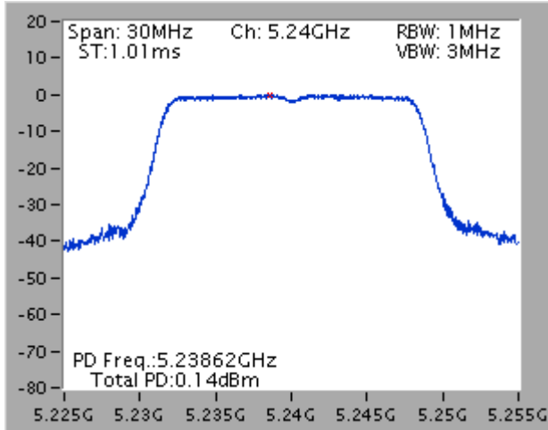
11a
