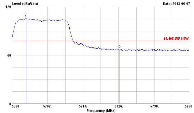
HT40,M8-15-(Highest Ch.)
