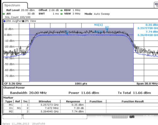
HT20 [Port 2]
