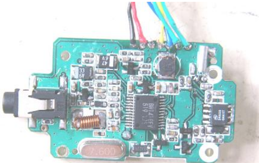
Main board component side
