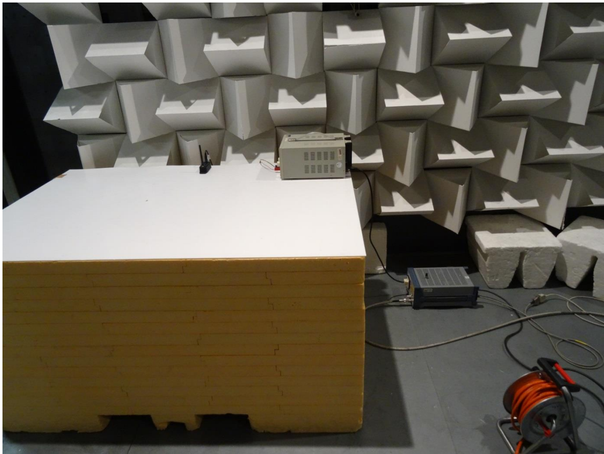
Conducted emission 150 kHz - 30 MHz
