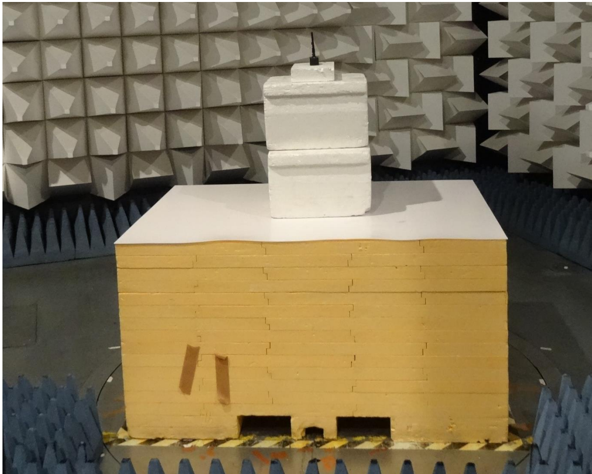
Radiated emission setup over 1GHz
