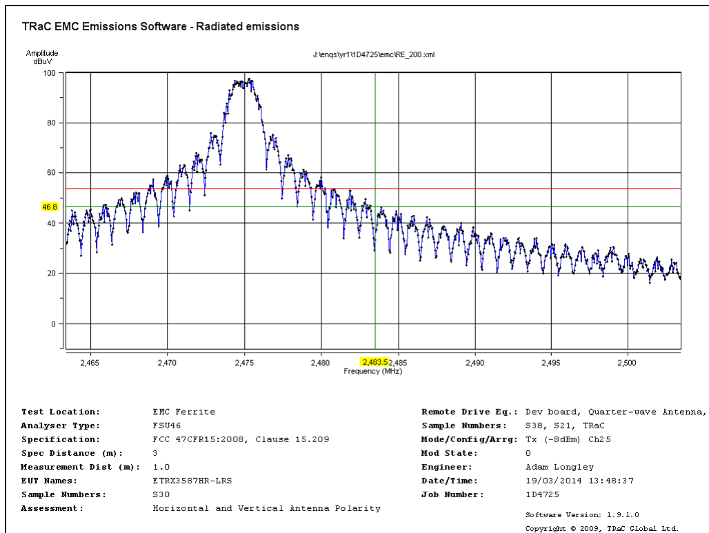
Radiated Transmitter Emissions Channel 25 2475MHz (15.209) Band Edge Compliance Band-Edge plot Quarter-wave Antenna
