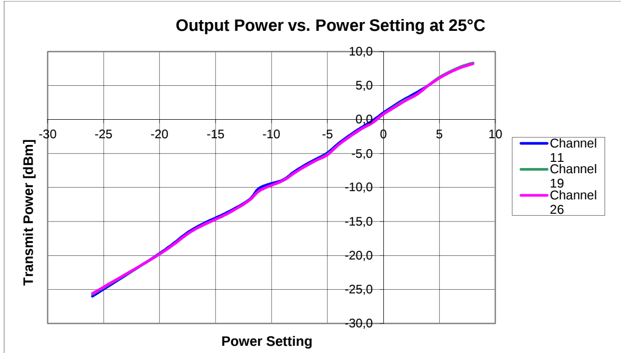
Figure 5.1 - Output Power vs. Power Setting
