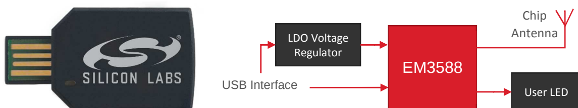
Figure 1.1 - Block Diagram
