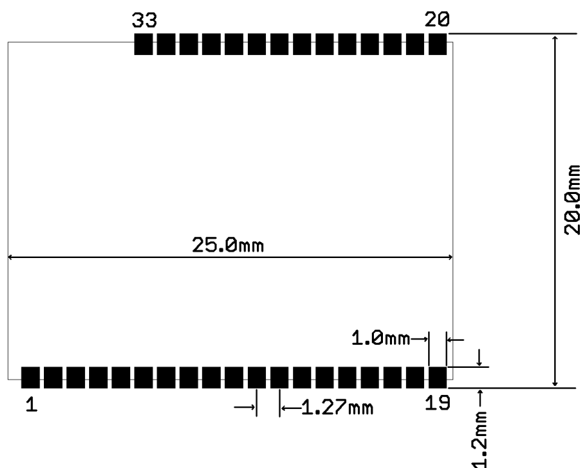
Figure 8: Recommended Footprint
