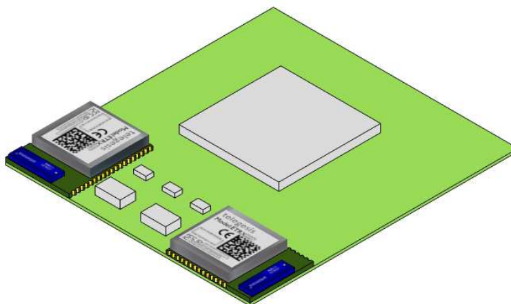
Figure 10. Typical placement
