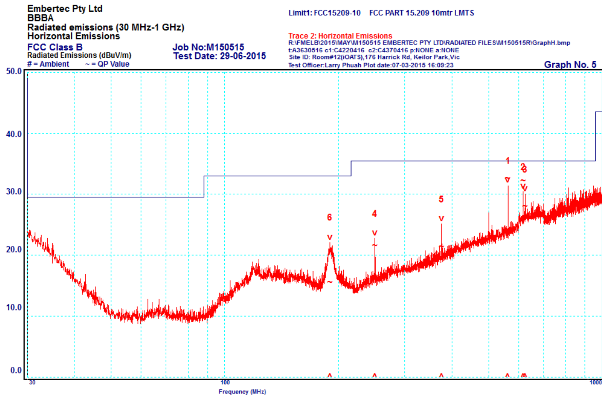
Graph 5: Horizontal Emissions 30 – 1000 MHz
