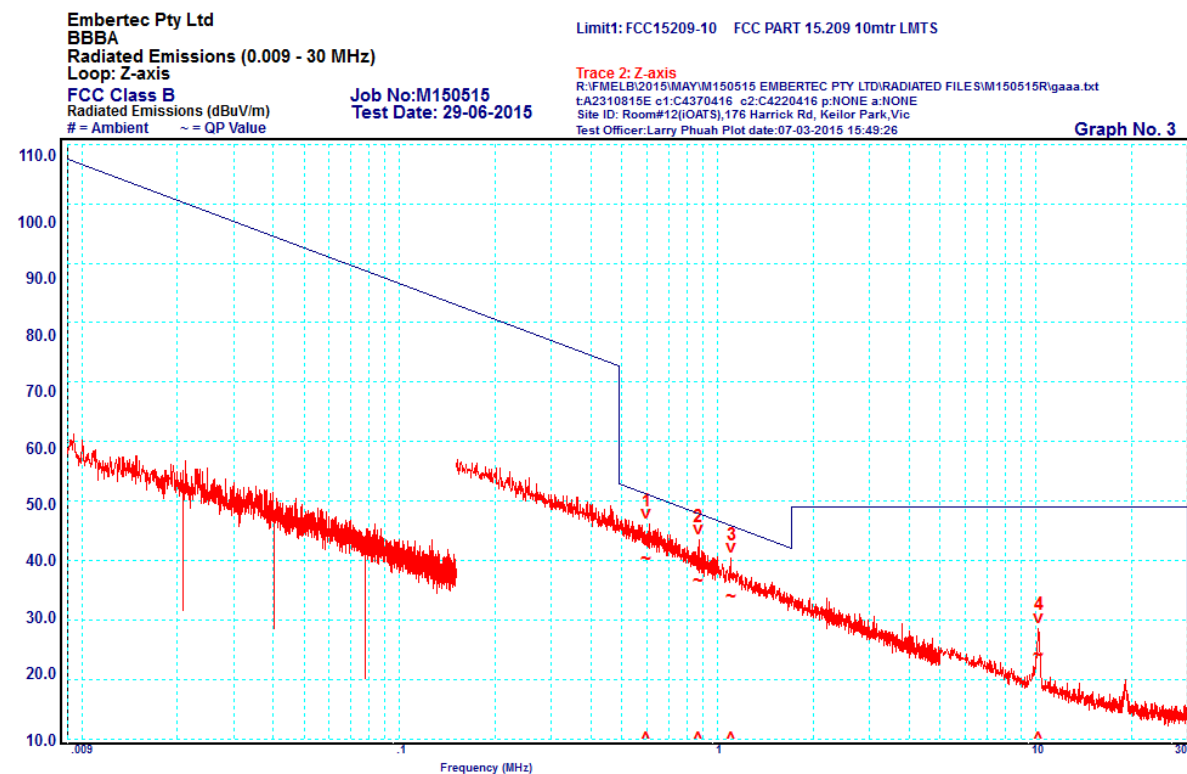
Graph 3: Loop: Z-Axis 9 kHz – 30 MHz
