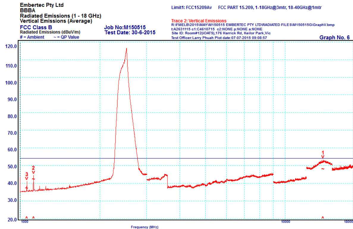
Graph 6: Vertical Polarity (average) 1 – 18 GHz
