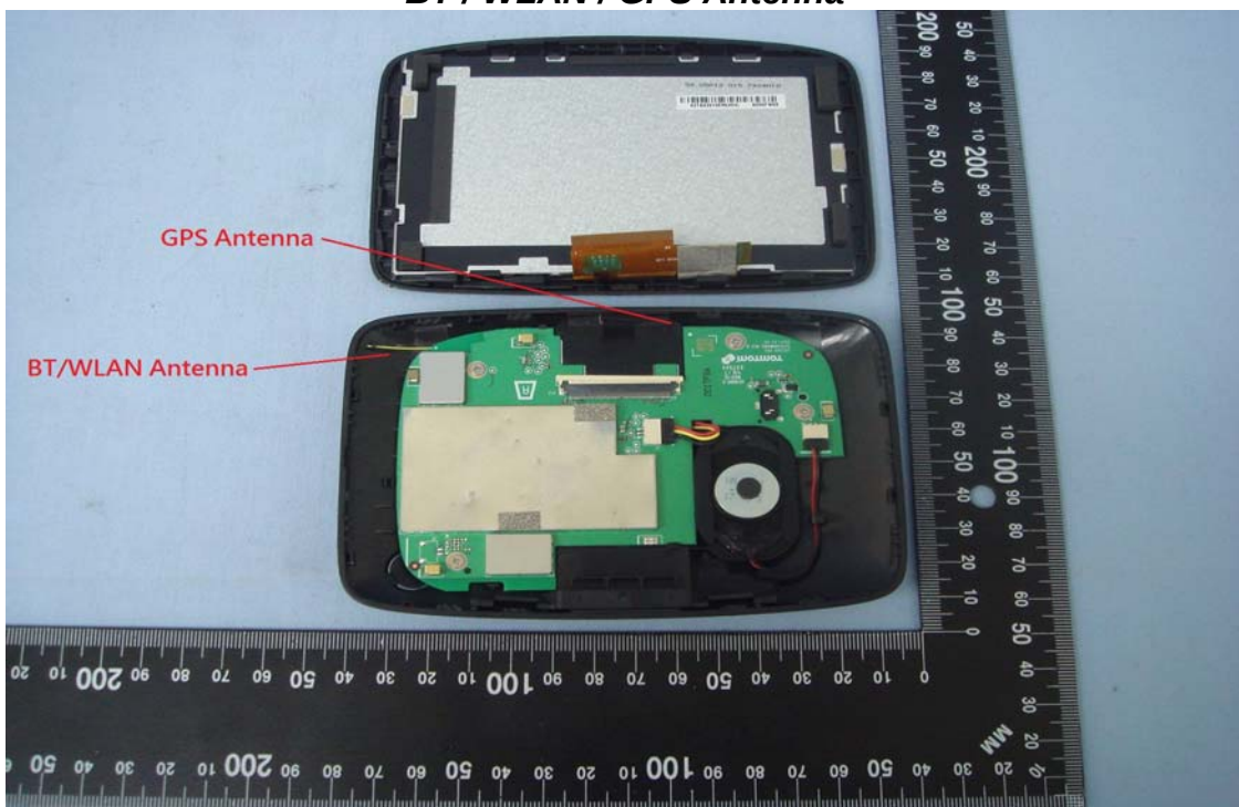
BT / WLAN / GPS Antenna
