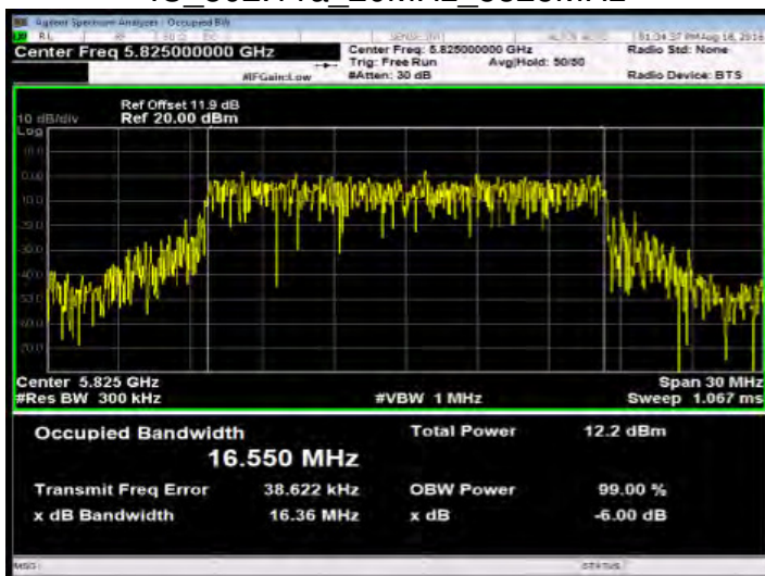
IC_802.11a_20MHz_5825MHz
