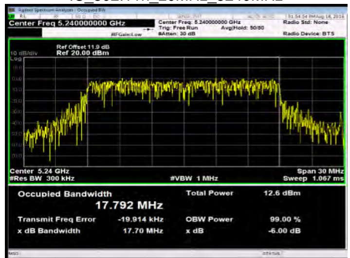
IC_802.11n_20MHz_5240MHz
