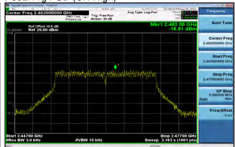
P802.11g PSD (CH-High)
