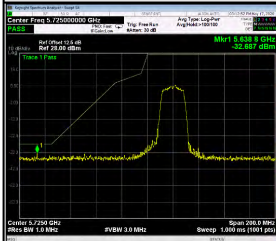
802.11n20 Left Side
