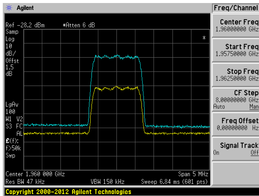
Downlink. Band 2 &amp; 25. CDMA
