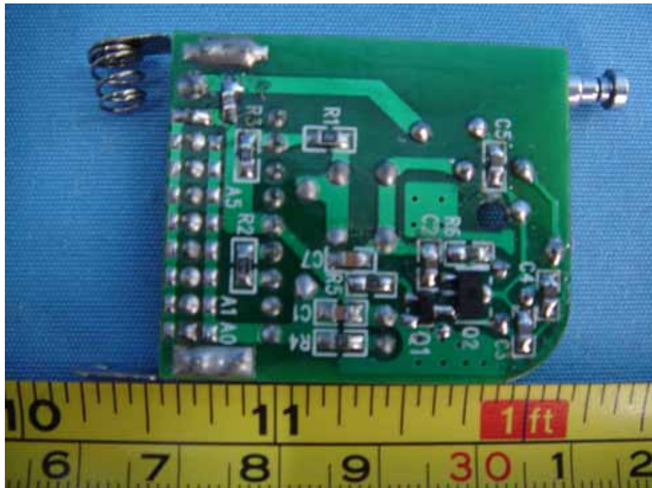
PCB - PCB - Solder View
