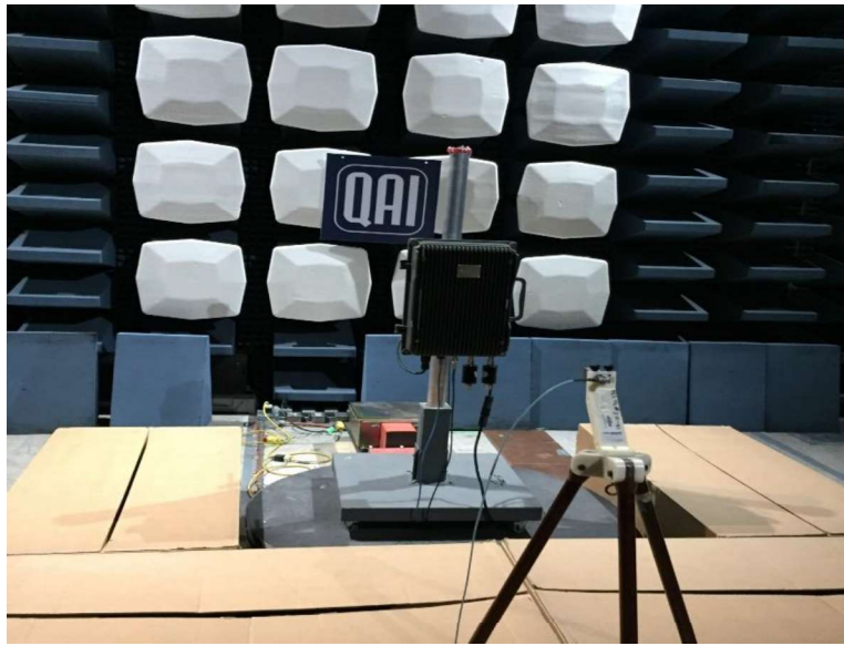
Figure 5: Radiated Emissions above 18GHz
