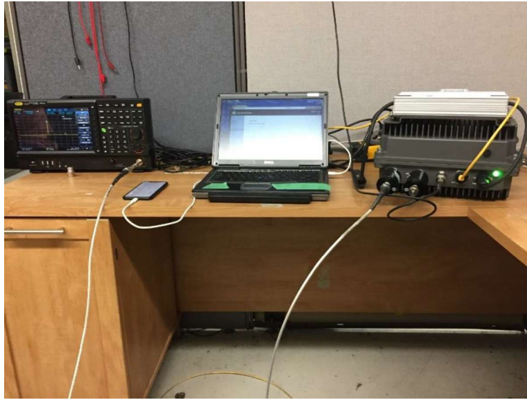
Figure 7: Radio Testing Station
