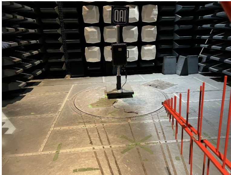
Figure 3: Radiated Emissions 30MHz. – 1GHz.
