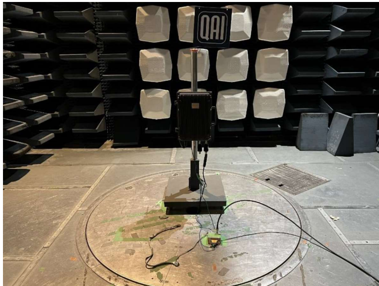
Figure 4: Conducted Emissions- Telecom
