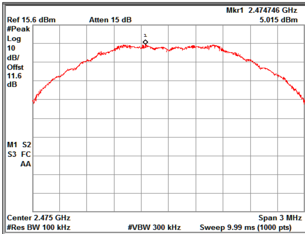
Reference plot for 2475MHz
