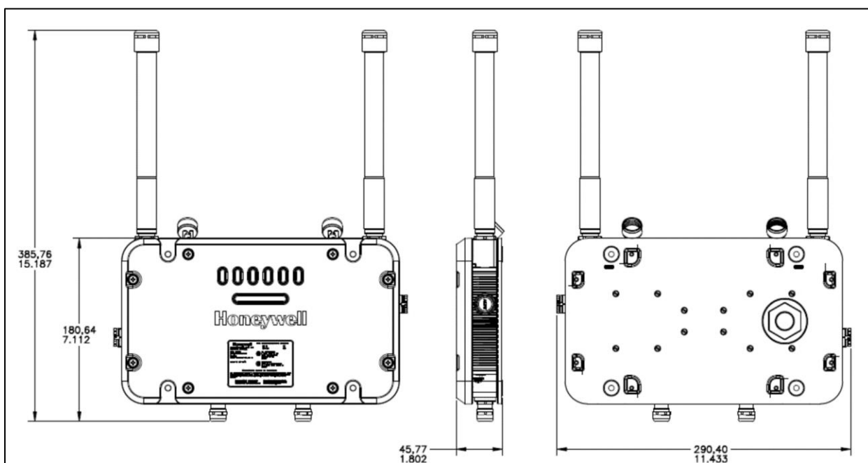
Fig. 31. FDAP Gen3 and FDAP Gen3 Anchor WITHOUT LIGHTENING SURGE ARRESTOR
