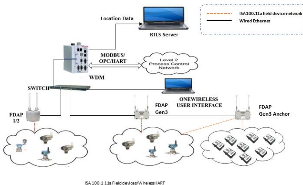
Fig. 1. OneWireless Network
