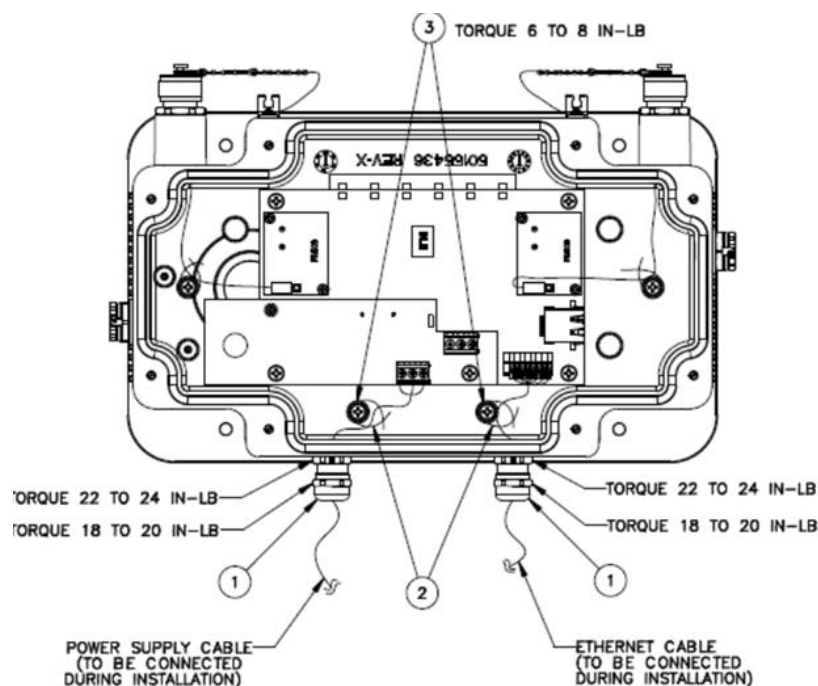
Fig. 14. FDAP Gen3 Ethernet and field DC power
