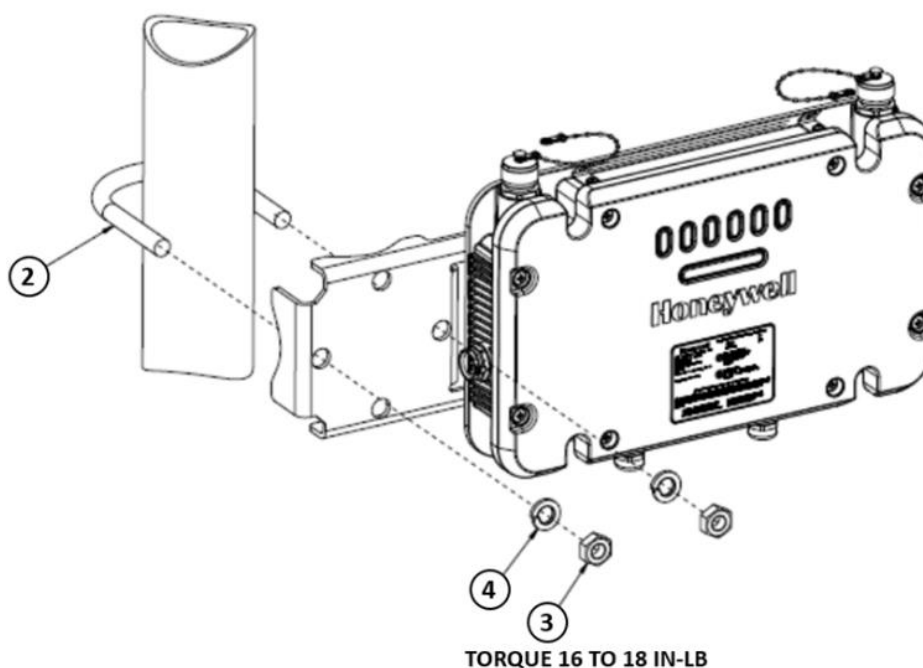
Fig. 10. Pole mounting of FDAP Gen3 and FDAP Gen3 Anchor
