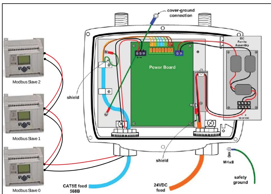
Fig. 28. FDAP2 Connection with Modbus
