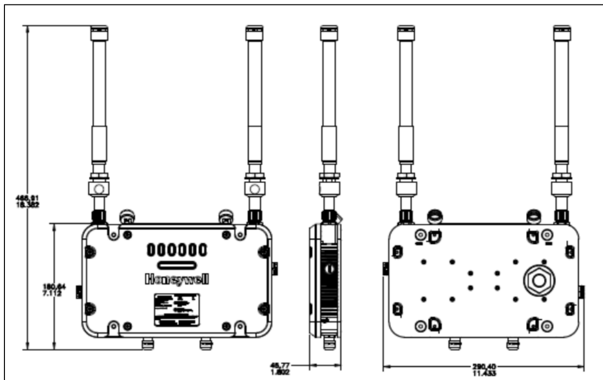
Fig. 30. FDAP Gen3 and FDAP Gen3 Anchor WITH LIGHTENING SURGE ARRESTOR
