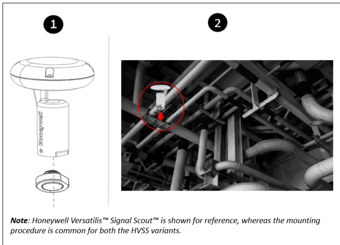
Figure 5-1: Magnetic Adapter Mounting
