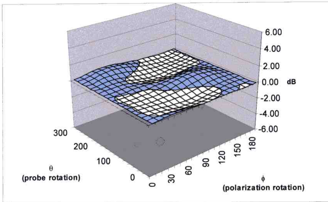
Surface Isotropy diagram of IXP-050 Probe S/N 0177 at 900MHz after VPM (rotational isotropy at side \pm 0.07 dB, spherical isotropy \pm 0.59 dB)
