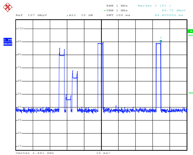
2DH5 on time (Count Pulses) Plot on Channel 39
