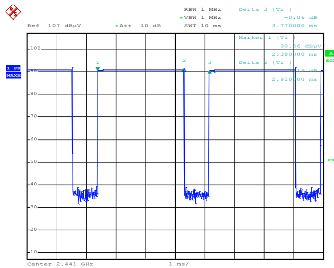
2DH5 on time (One Pulse) Plot on Channel 39
