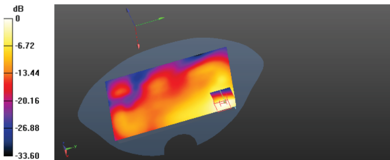
Figure 6 : Body, Rear Side, WCDMA Band II Channel 9400
