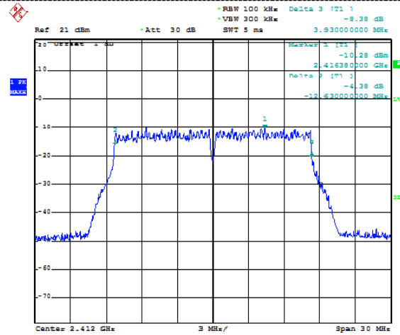
802.11g
