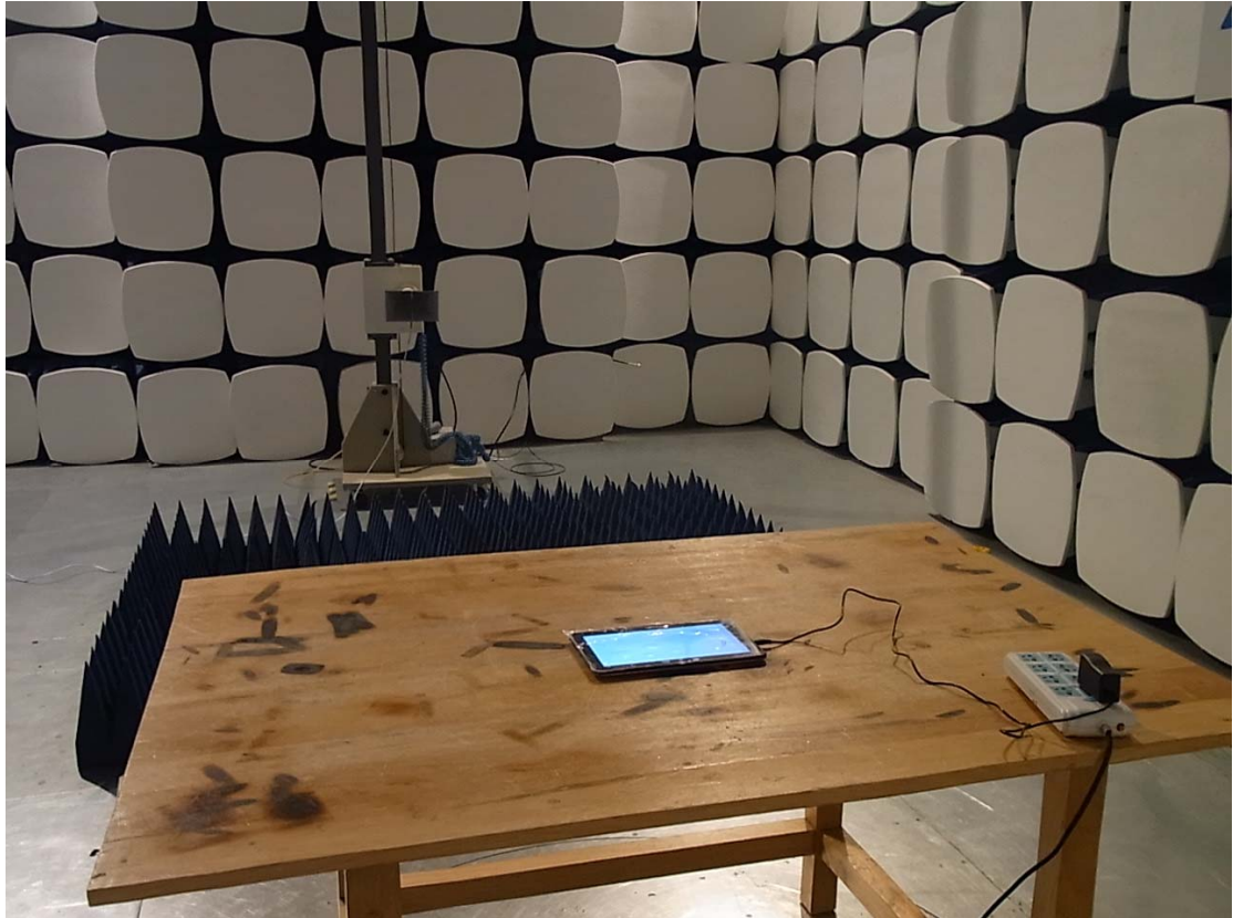
Radiated Emission (1GHz-25GHz)
