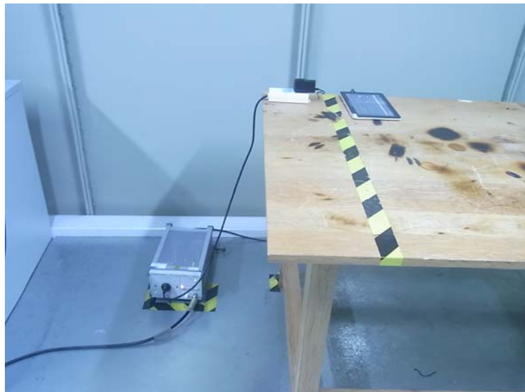
Conducted Emission
