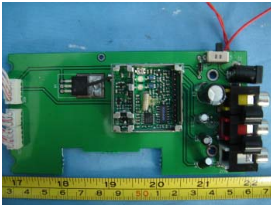
PCB - Component View (1.1)
