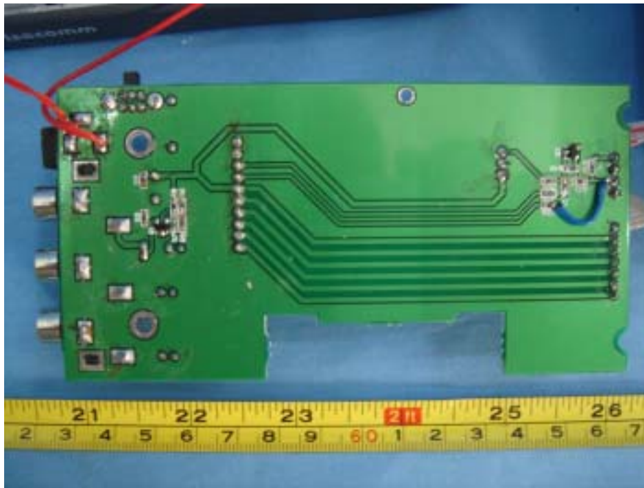
PCB - Solder View(1)
