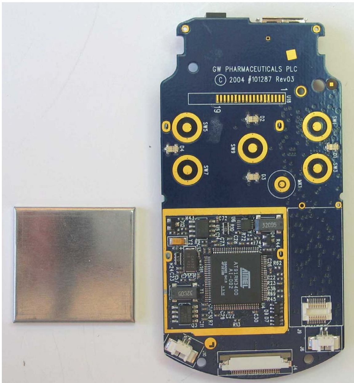
Top Side of Board
