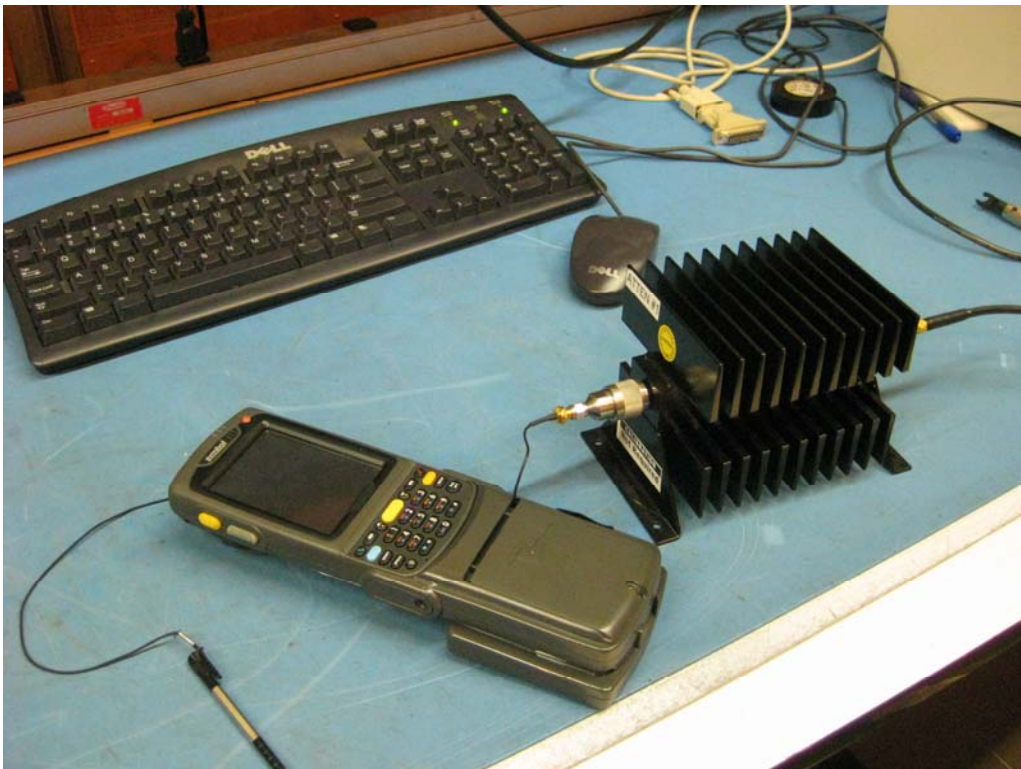
Conducted RF #2
