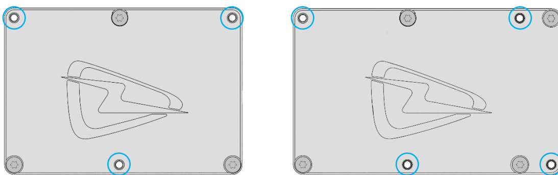
Figure 1 - position of mounting points (left – 3117, right – 3417/3419)
