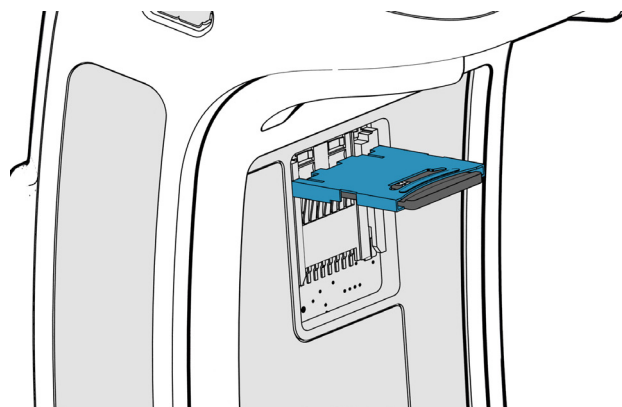
FIGURE 13: MicroSD inserted correctly
