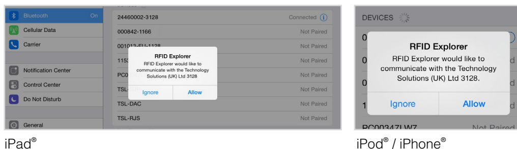
Figure 25: Allow connection
