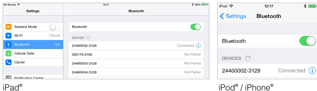
Figure 24: Device connected
