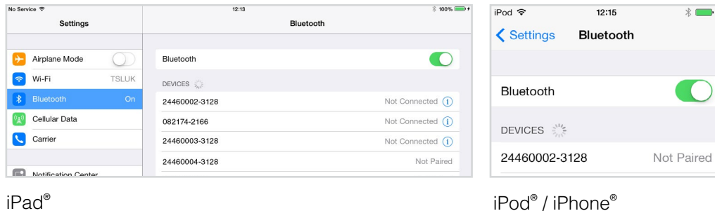
Figure 23: Identify device
