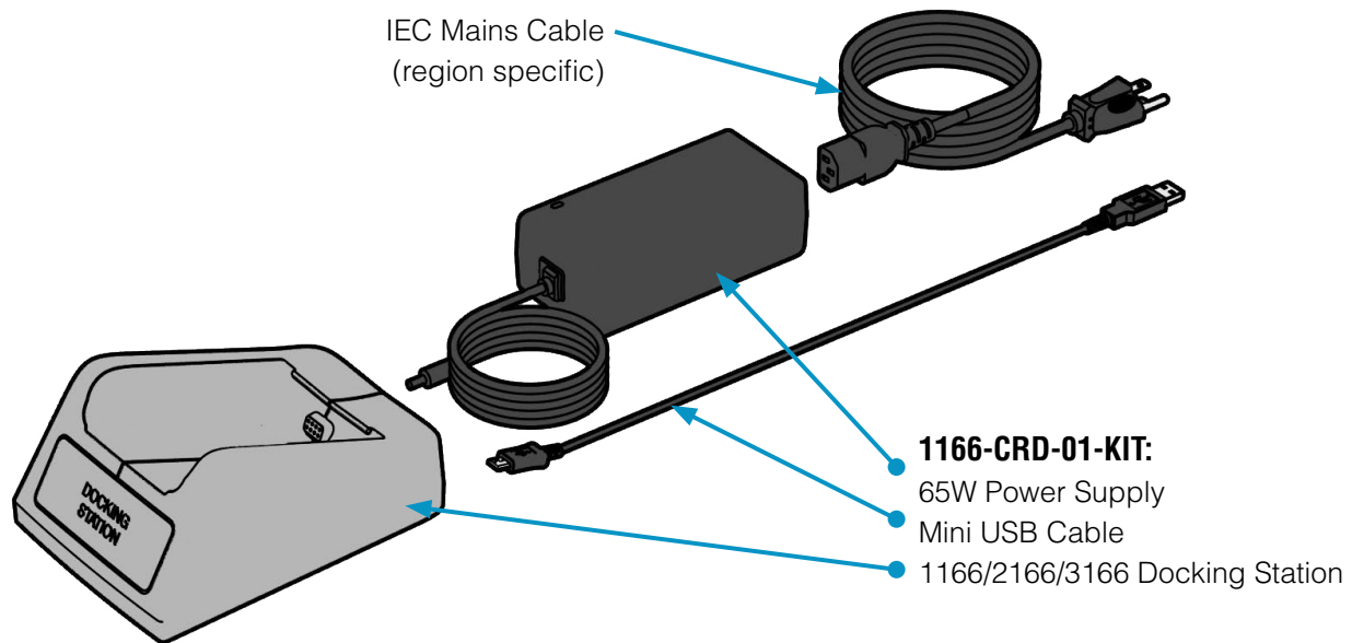
Figure 4: Components required for charging the 3166 UHF Reader
