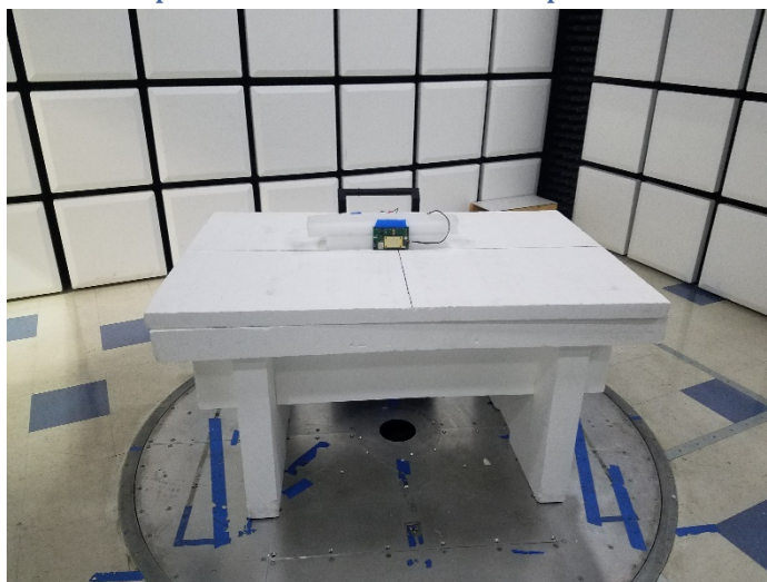
Radiated Output Power and Radiated Spurious Emissions
