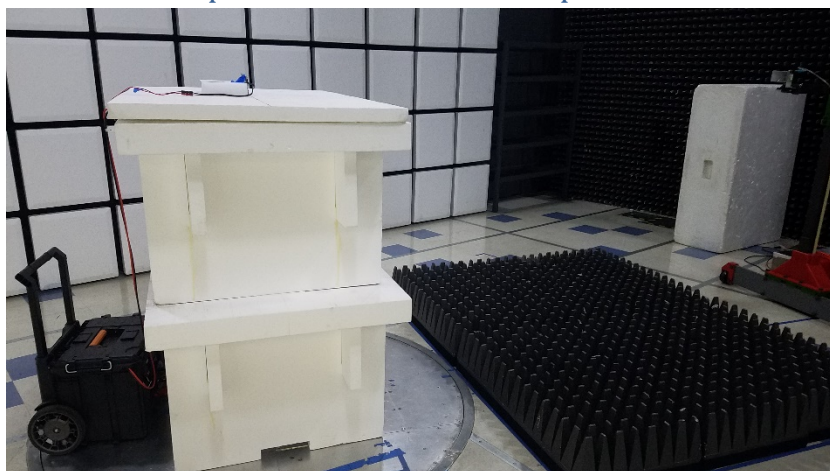
Radiated Output Power and Radiated Spurious Emissions
