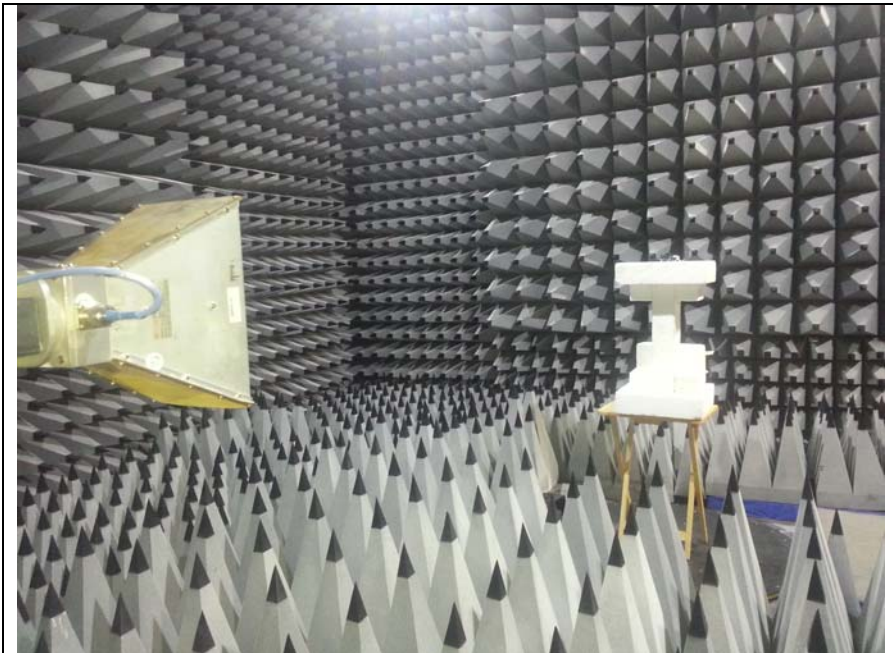
Fig 3 Test setup 1GHz -9.2GHz Rad Emission
