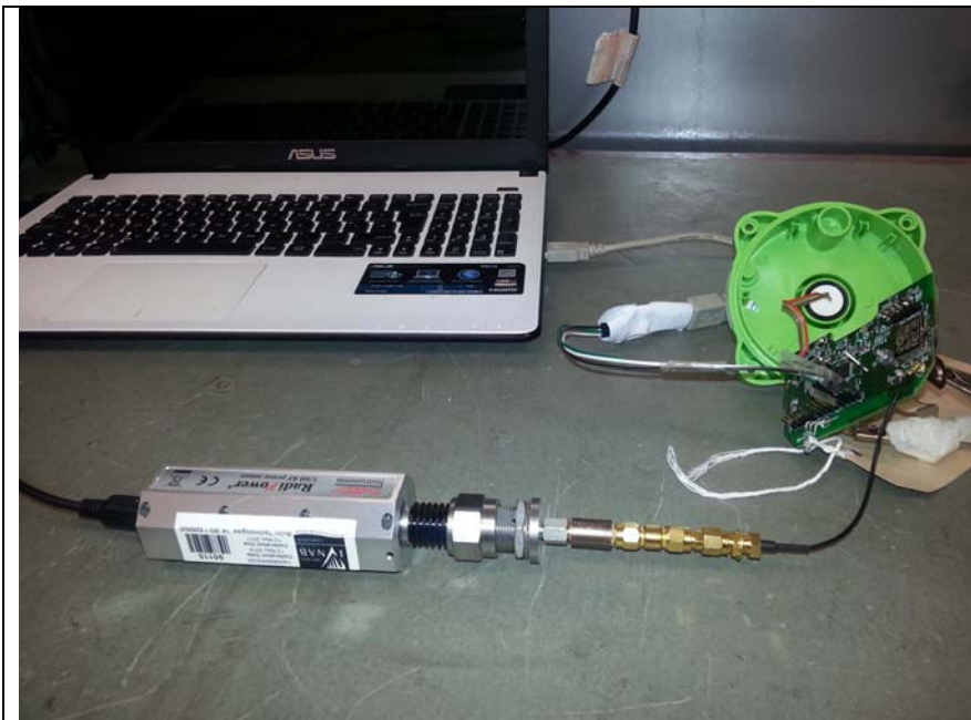
Fig 4 Test setup Conducted Emissions
