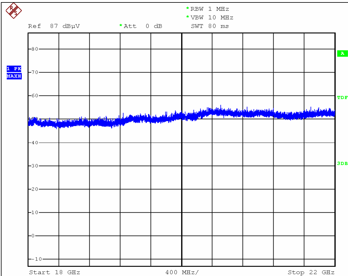
Fig C13 Low Channel Radiated Emissions 18GHz -22GHz Vertical 1 metre
