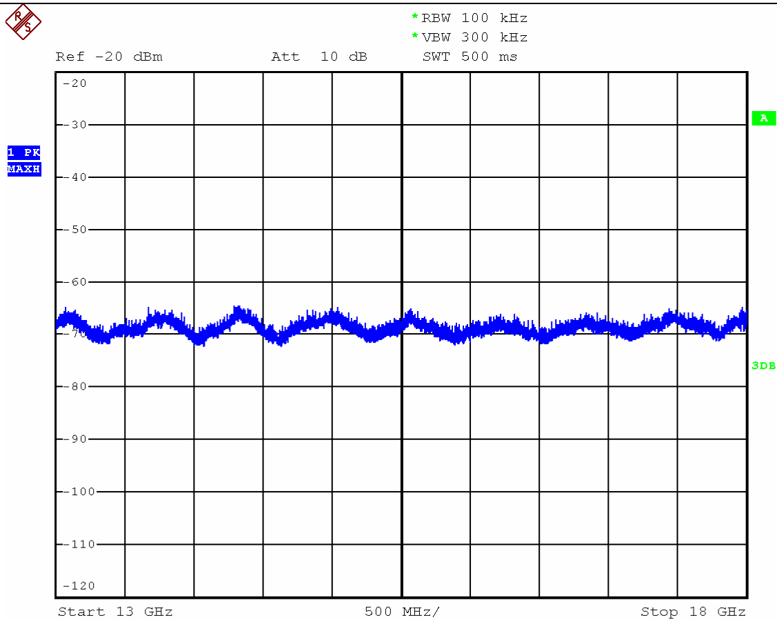
Fig A6 Low Channel Conducted Spurious Emissions 13GHz -18GHz
