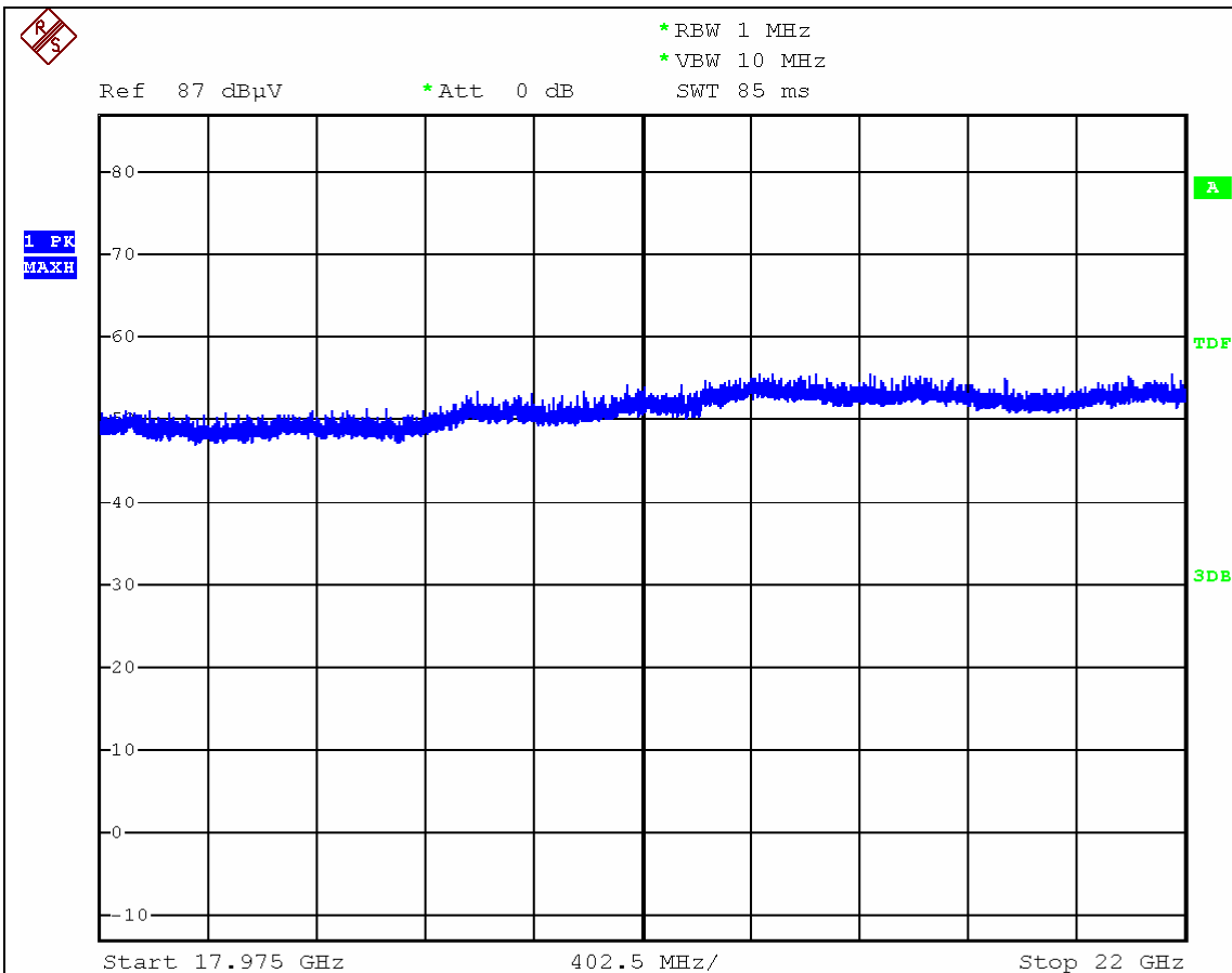
Fig C14 Low Channel Radiated Emissions 18GHz -22GHz Horizontal 1metre
