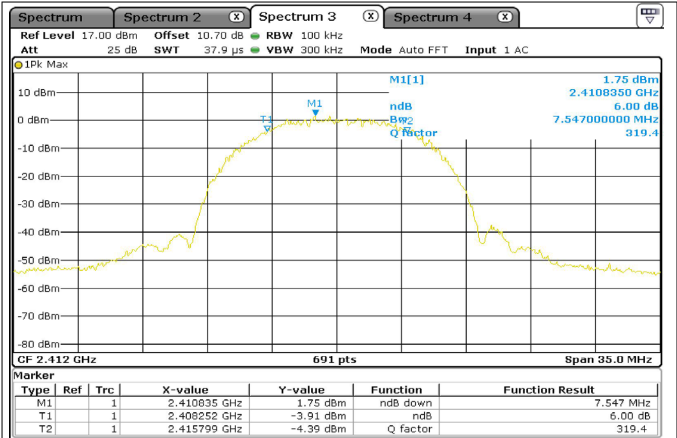
Fig 1 6dB Bandwidth
