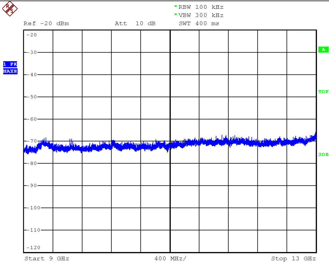
Fig A5 Low Channel Conducted Spurious Emissions 9 GHz -13GHz
