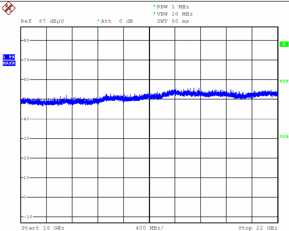
Fig D13 Low Channel Radiated Emissions 18GHz -22GHz Vertical 1 metre
