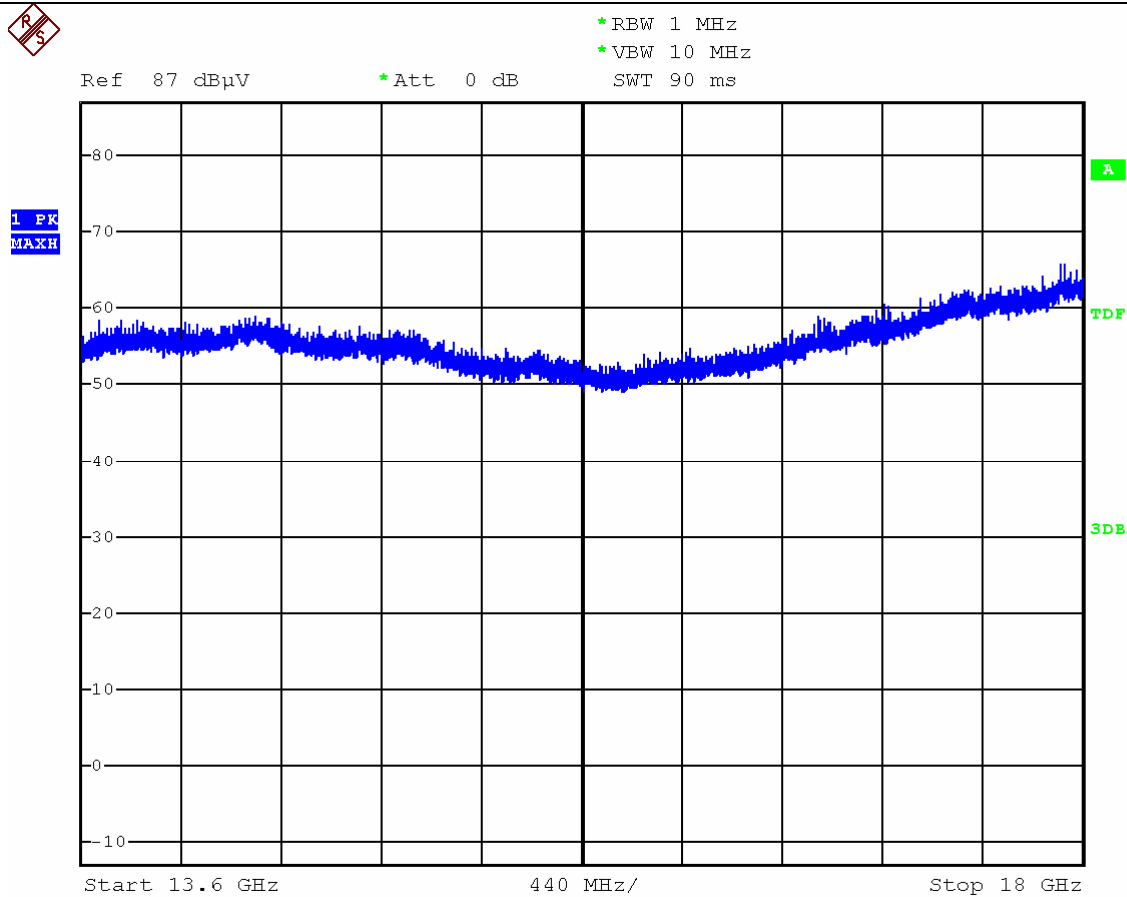
Fig D11 Low Channel Radiated Emissions 13.6GHz -18GHz Vertical 1 metre
