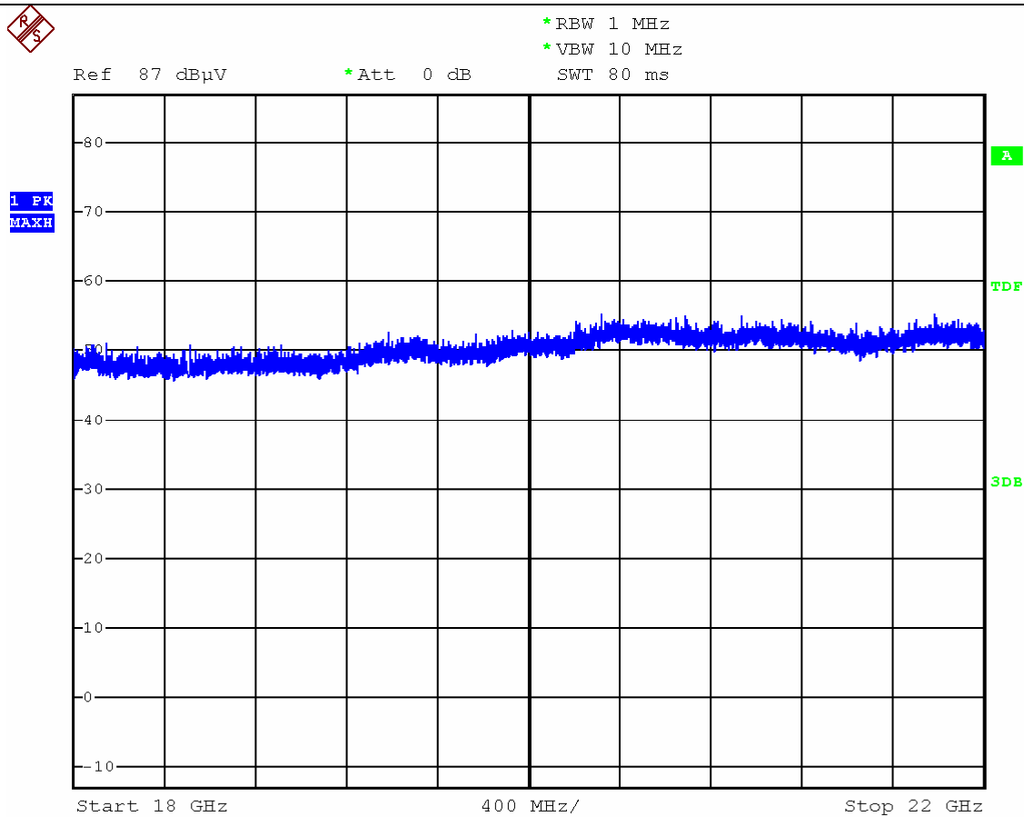
Fig D14 Low Channel Radiated Emissions 18GHz -22GHz Horizontal 1metre
