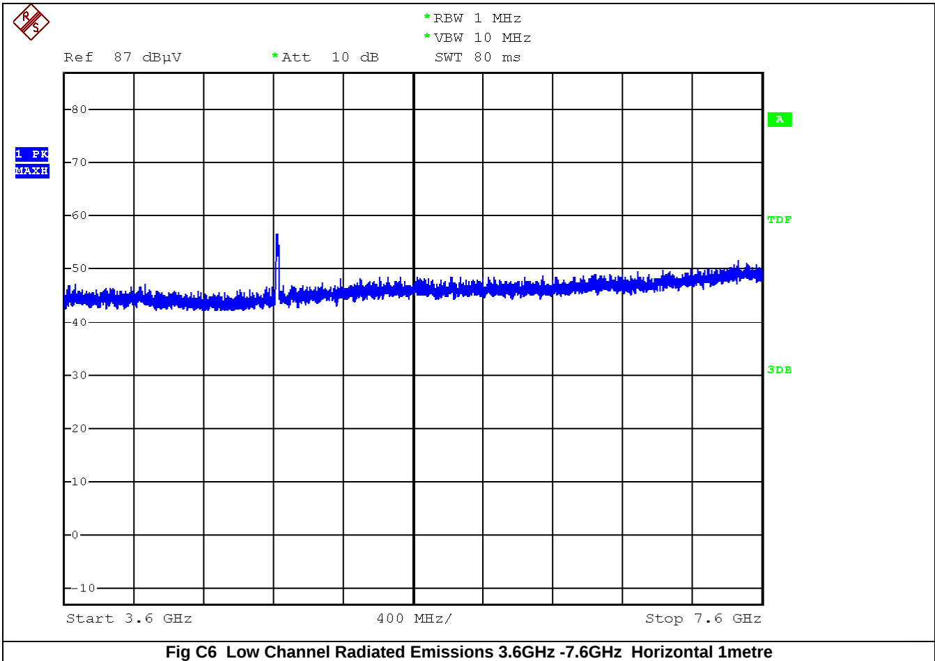
Fig C6 Low Channel Radiated Emissions 3.6GHz -7.6GHz Horizontal 1metre
