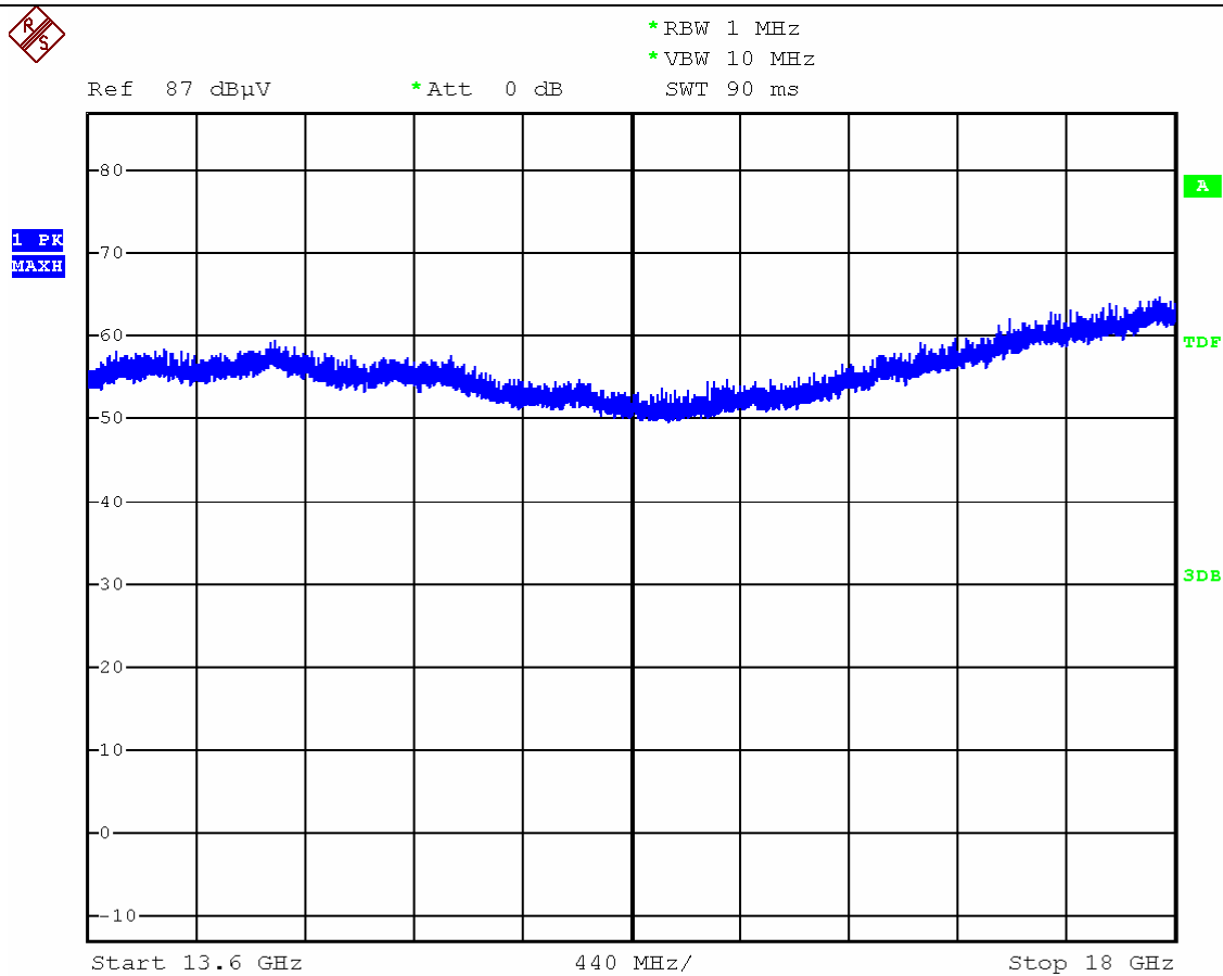
Fig D12 Low Channel Radiated Emissions 13GHz -18GHz Horizontal 1metre
