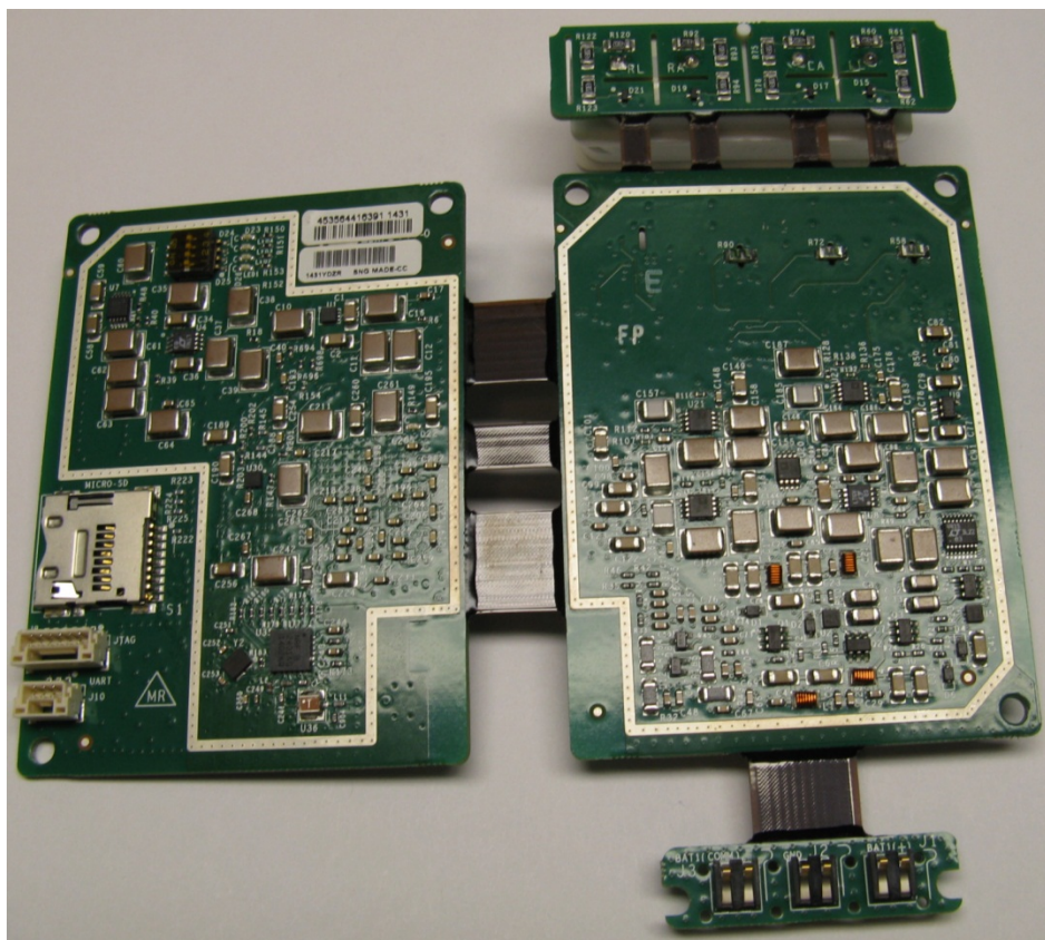
wECG – Bottom (Metal Cover Removed)
