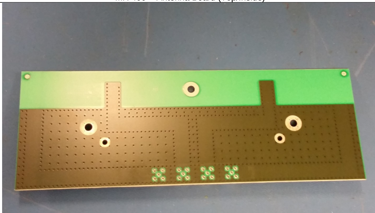
MR400 - Antenna Board (Bottom/Outside)
