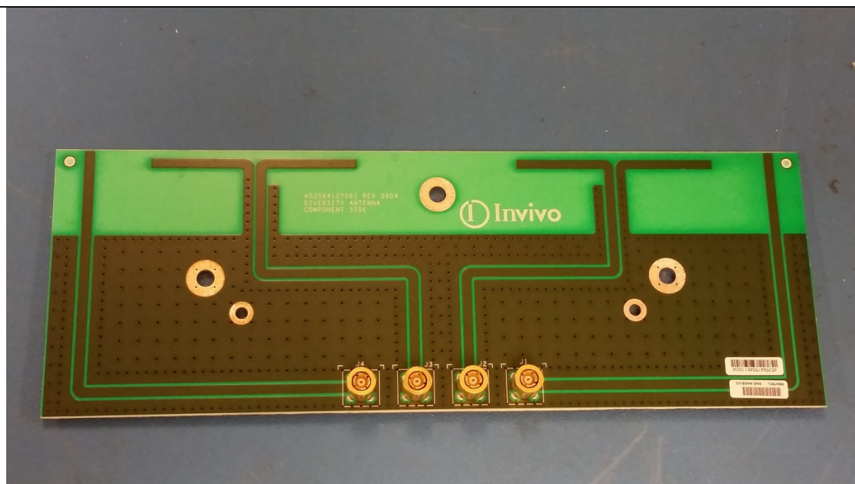
MR 400 - Antenna Board (Top/Inside)
