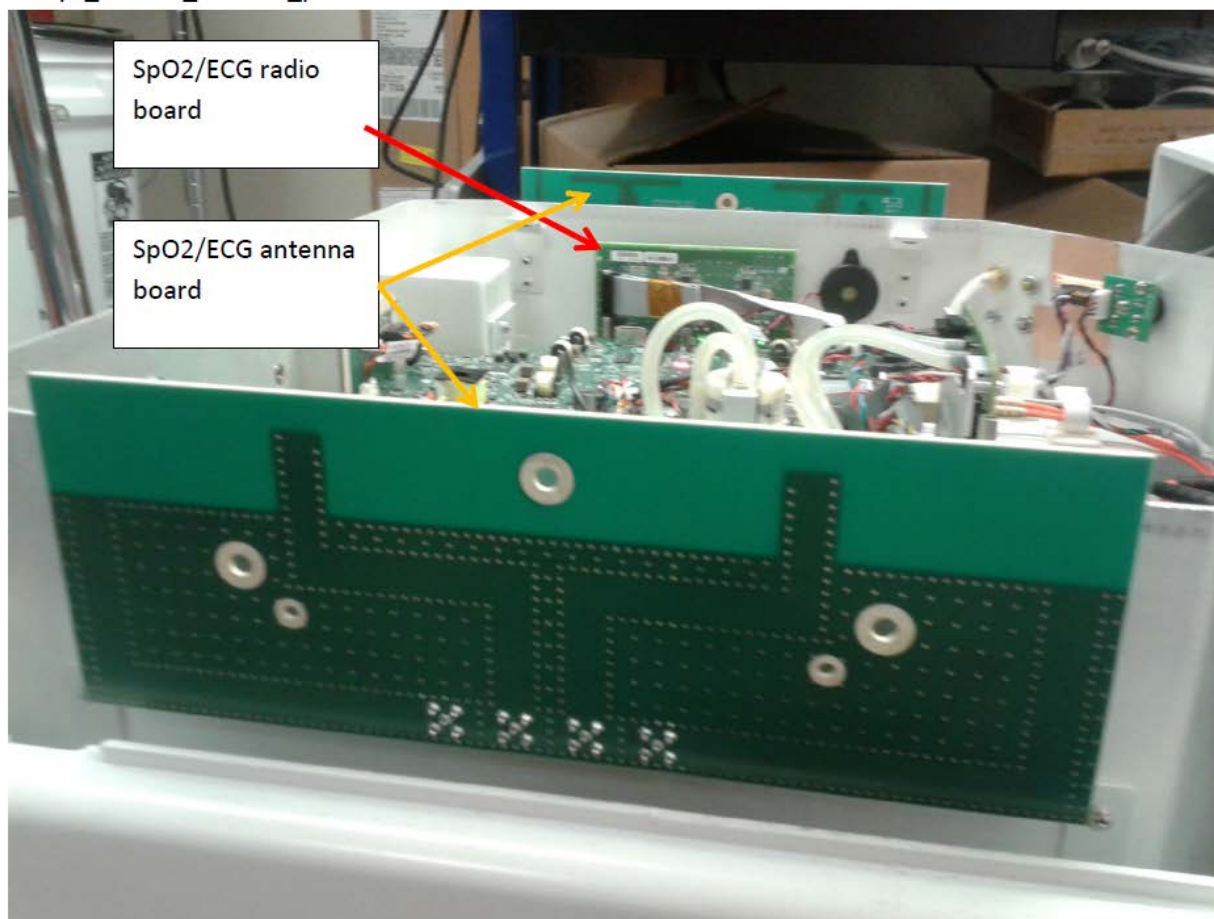
MR400 – Overall Interior
