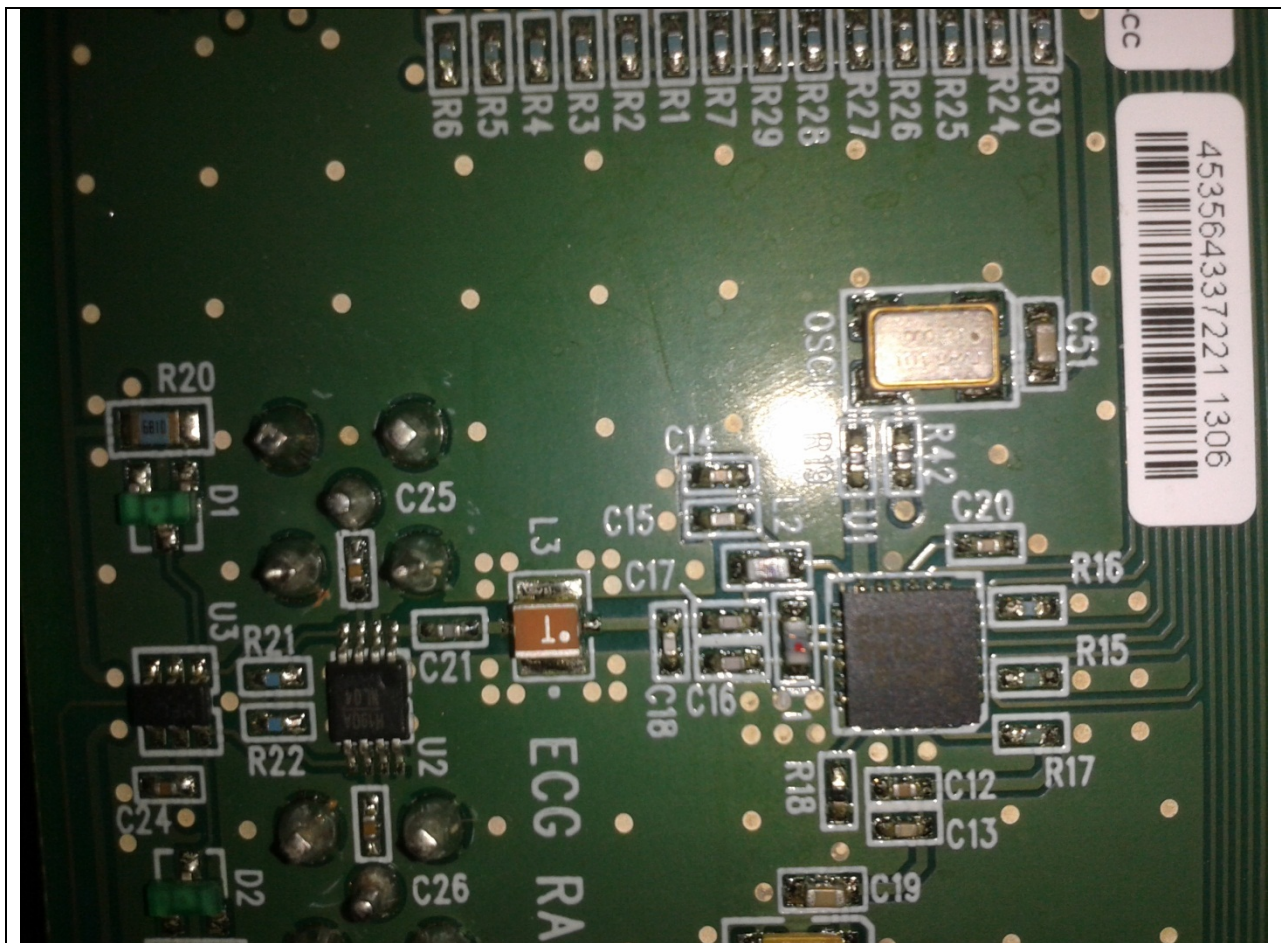
MR 400 - Radio Board (ECG Zoomed In)
