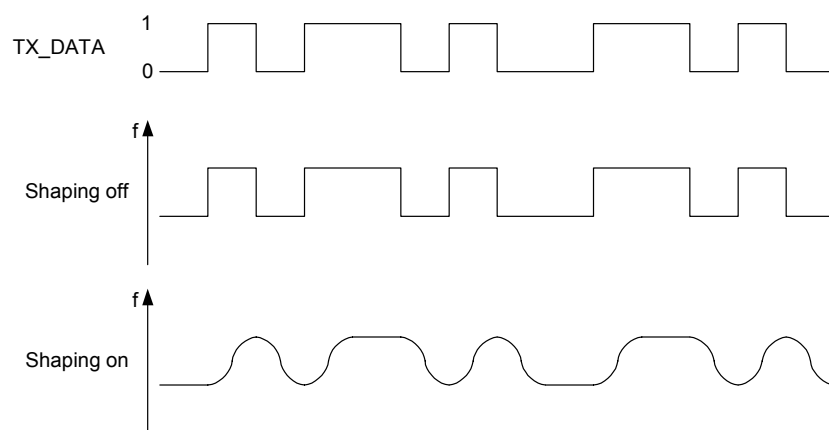
Figure 23. FSK spectrum shaping by smooth frequency transitions
