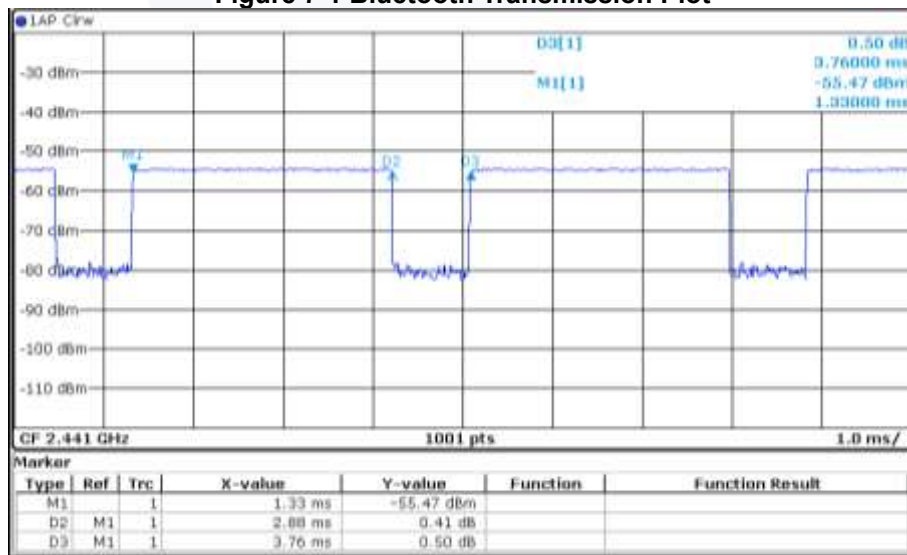
Figure 7-1 Bluetooth Transmission Plot
