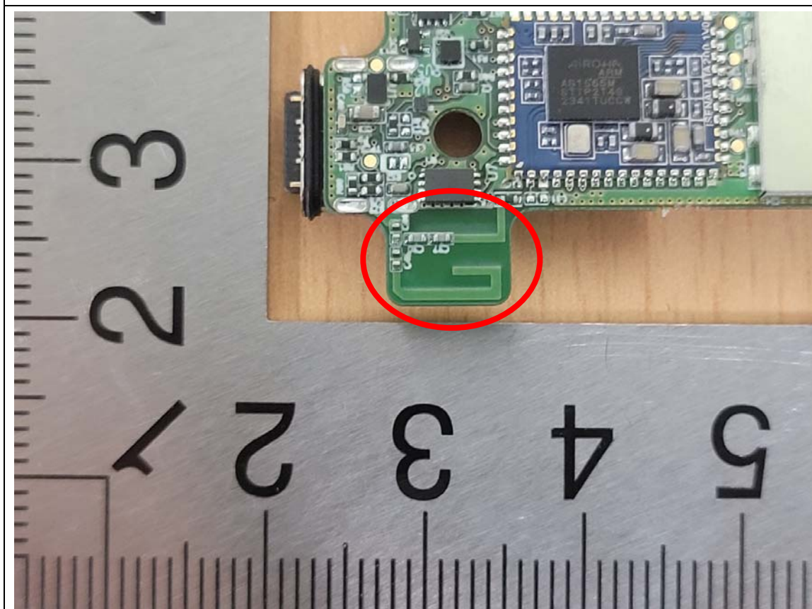
BT Antenna
