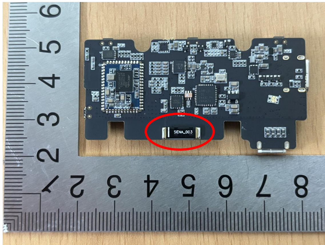
MESH Antenna
