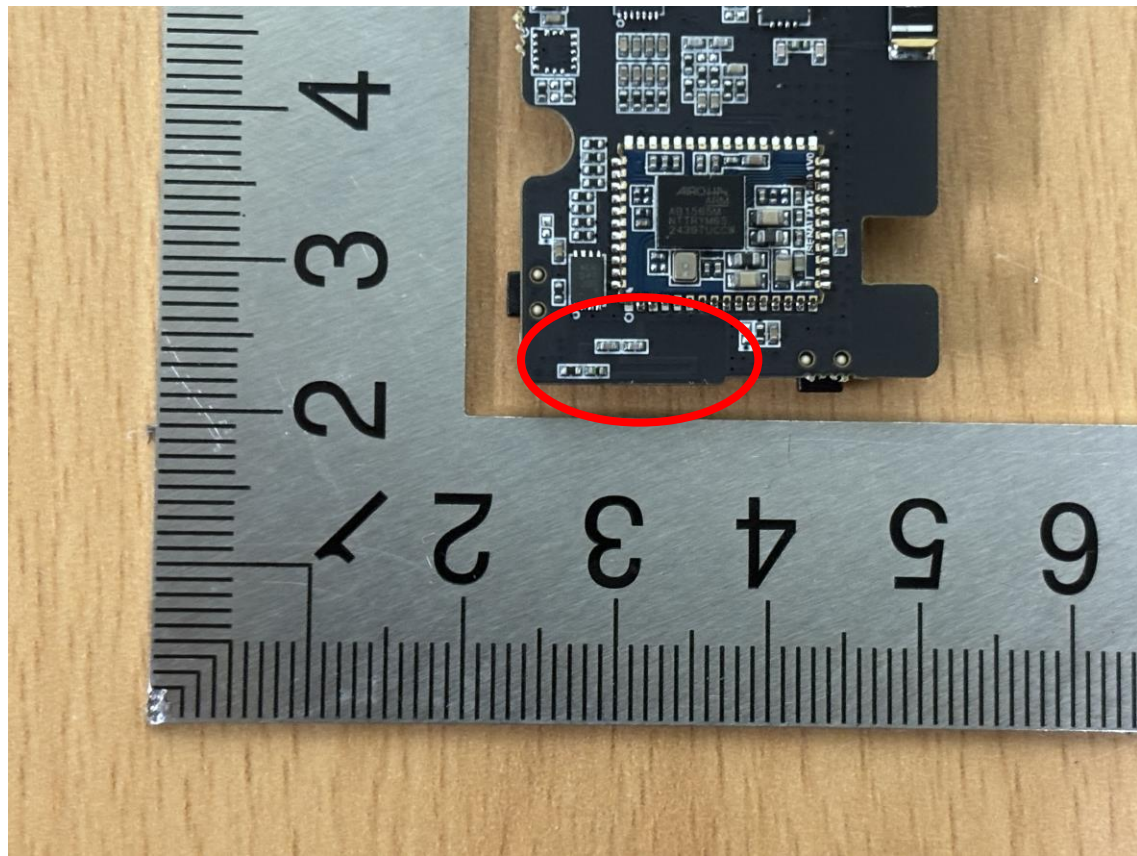
BT Antenna
