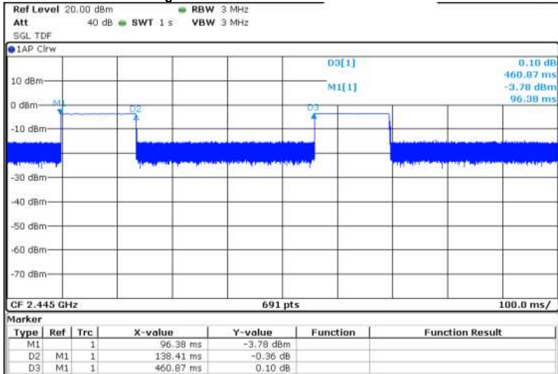
Figure 7-1 MESH Ant.2 Transmission Plot
