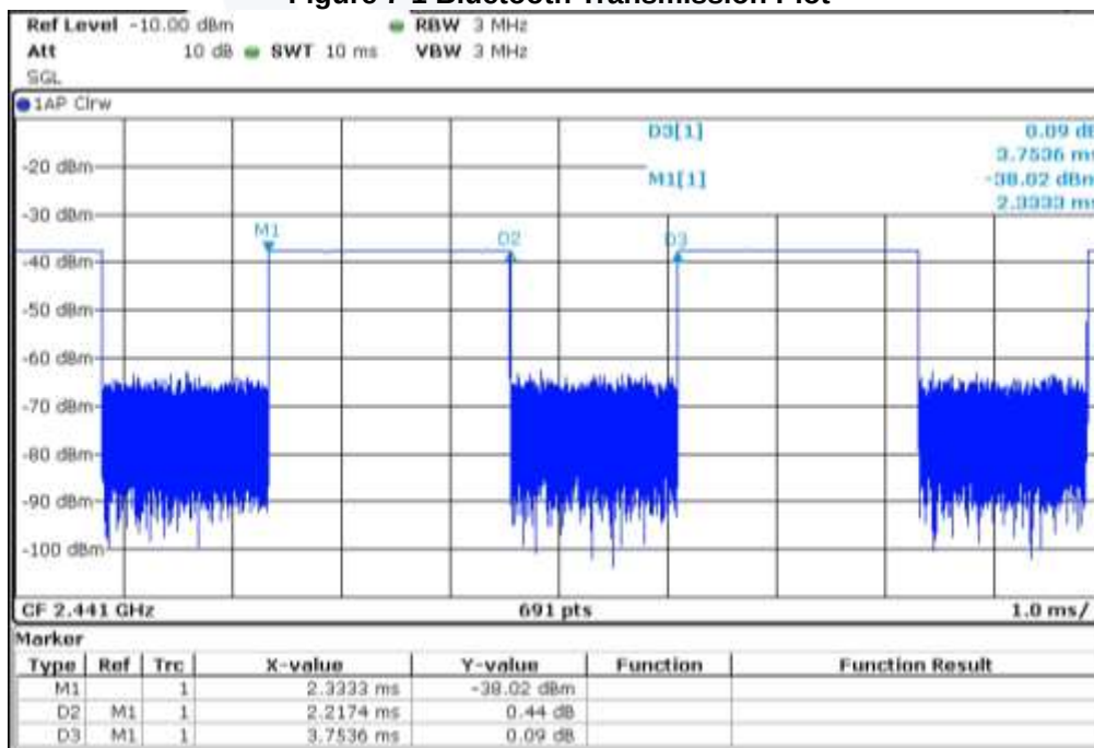
Figure 7-1 Bluetooth Transmission Plot
